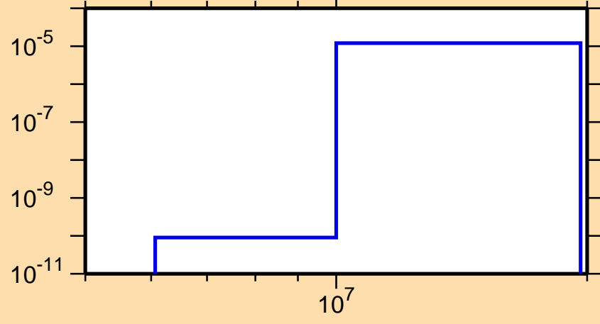
\sigma vs. E for ^{155}\text{Sm}(n,\alpha)
