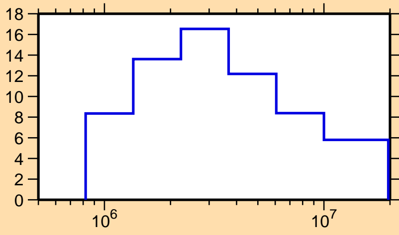
\Delta\sigma/\sigma vs. E for ^{155}\text{Sm}(n, el.)
