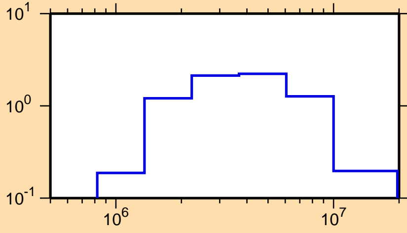
\sigma vs. E for ^{155}\text{Sm}(n,n\text{cont.})
