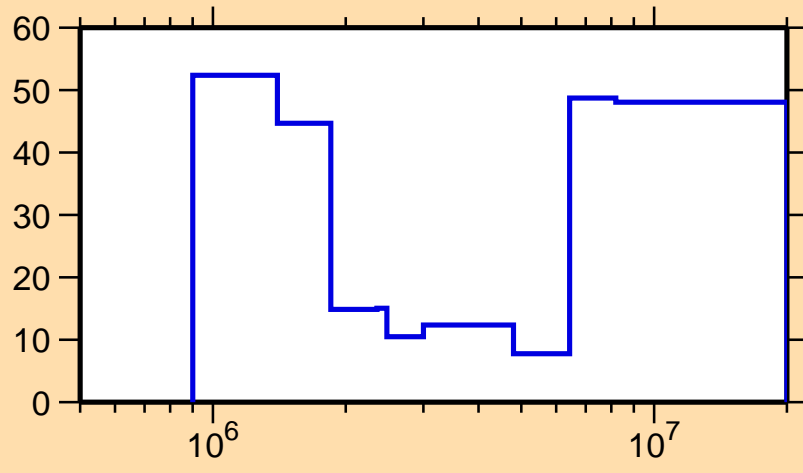
\Delta\sigma/\sigma vs. E for ^{155}\text{Sm}(n,n\text{cont.})
