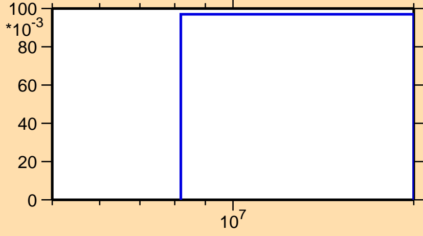
\sigma vs. E for ^{155}\text{Sm}(n,3n)
