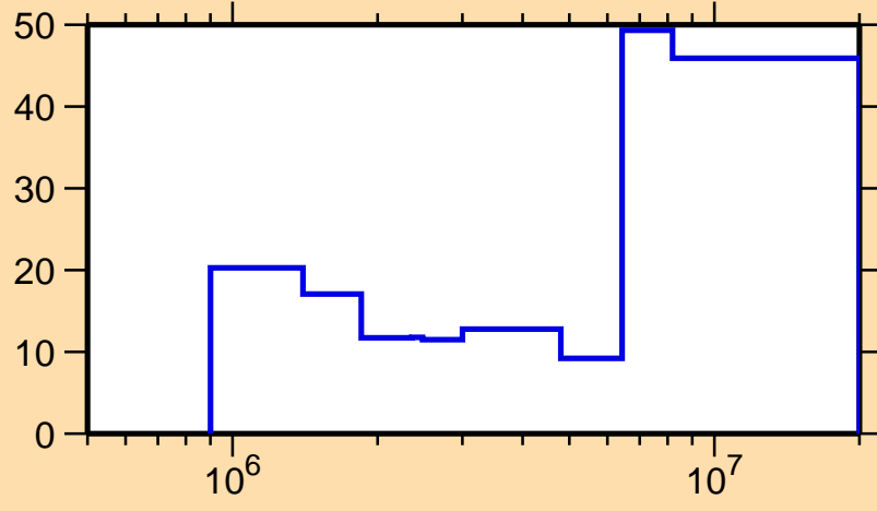
\Delta\sigma/\sigma vs. E for ^{155}\text{Sm}(n,\text{inel.})
