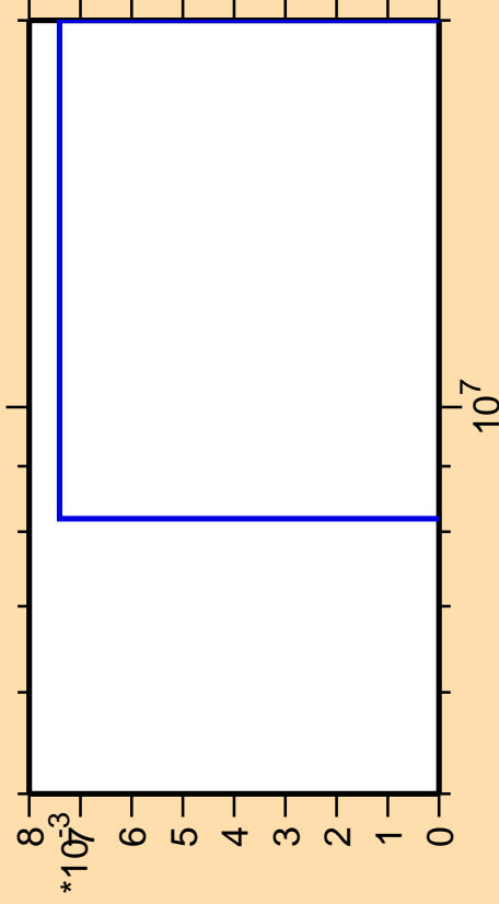
\Delta\sigma/\sigma vs. E for ^{155}\text{Sm}(n,\text{He}3)
