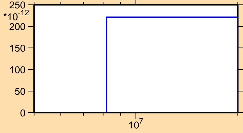
\sigma vs. E for ^{155}\text{Sm}(n,2np)
