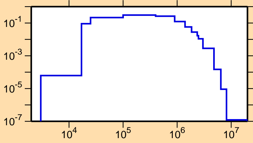
\sigma vs. E for ^{155}\text{Sm}(n,n_1)
