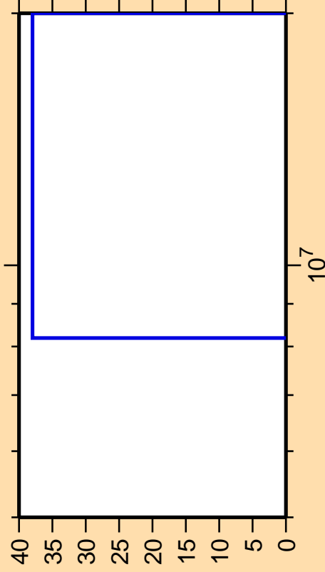
\Delta\sigma/\sigma vs. E for ^{155}\text{Sm}(n,3n)
