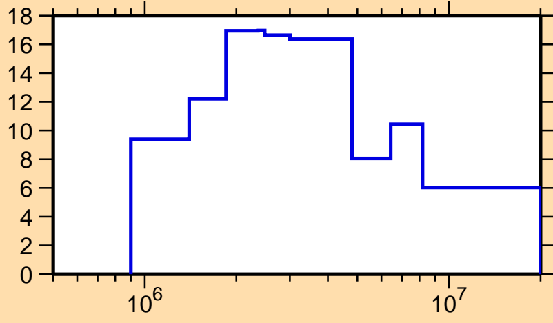
\Delta\sigma/\sigma vs. E for ^{155}\text{Sm}(n,\text{el.})
