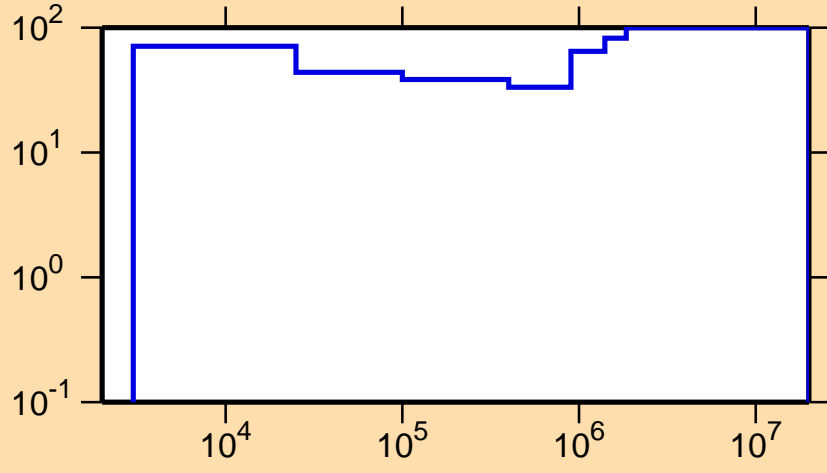
\Delta\sigma/\sigma vs. E for ^{155}\text{Sm}(n,n_1)
