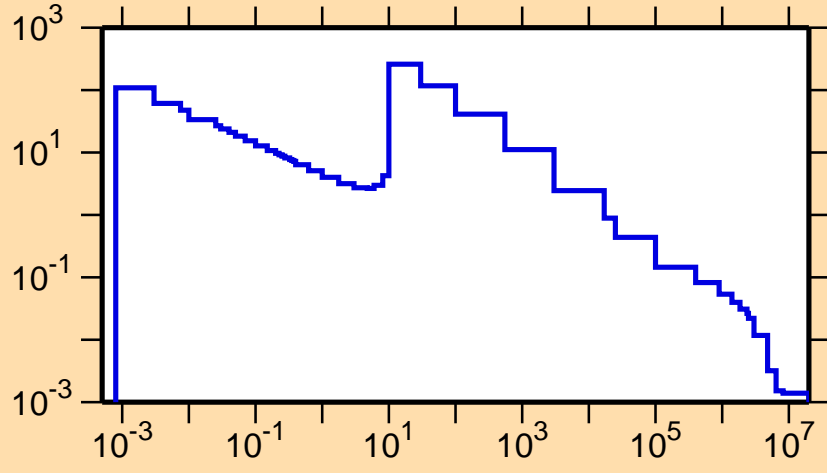
\sigma vs. E for ^{155}\text{Sm}(n,\gamma)
