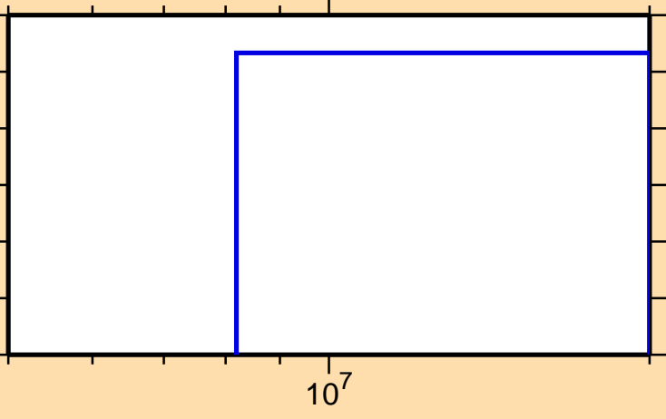
\sigma vs. E for ^{155}\text{Sm}(n,\text{nd})
