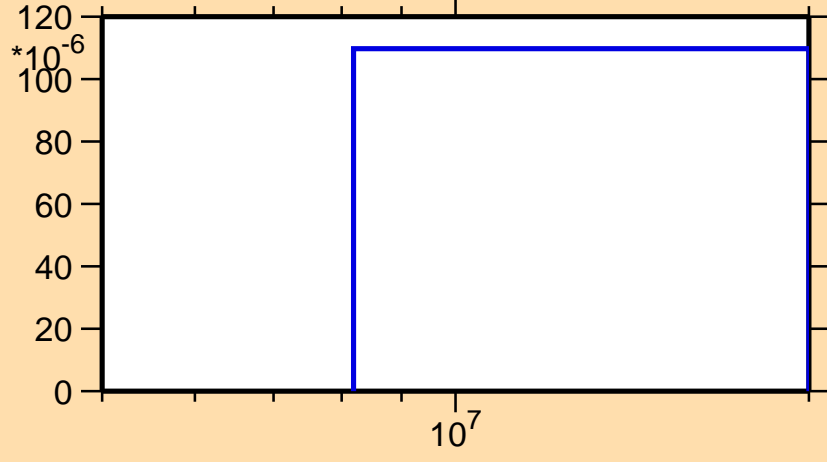
\sigma vs. E for ^{155}\text{Sm}(n,d)
