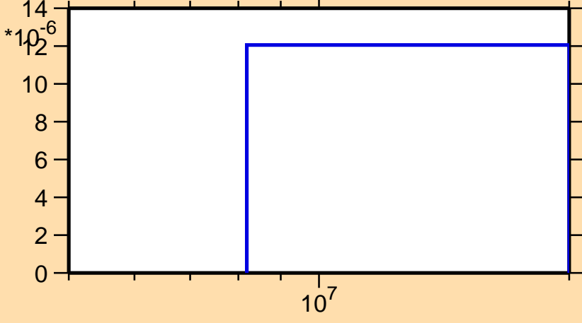
\sigma vs. E for ^{155}\text{Sm}(n,t)
