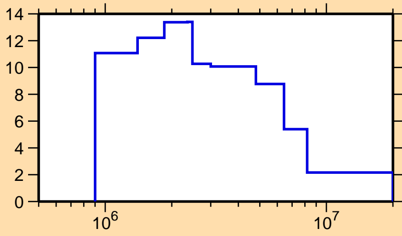
\Delta\sigma/\sigma vs. E for ^{155}\text{Sm}(n,\text{tot.})
