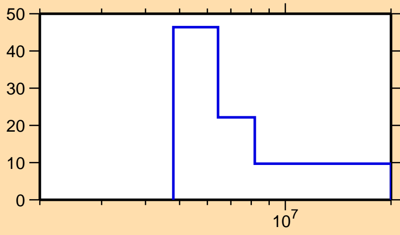
\Delta\sigma/\sigma vs. E for ^{155}\text{Sm}(n,2n)
