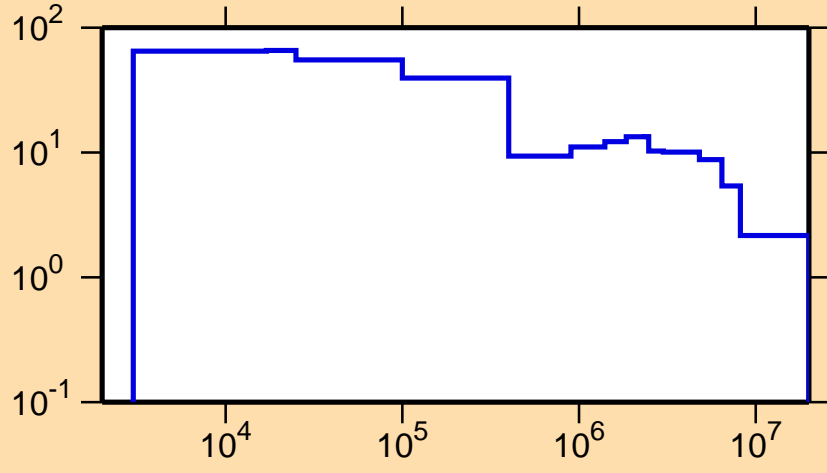
\Delta\sigma/\sigma vs. E for ^{155}\text{Sm}(n,\text{tot.})
