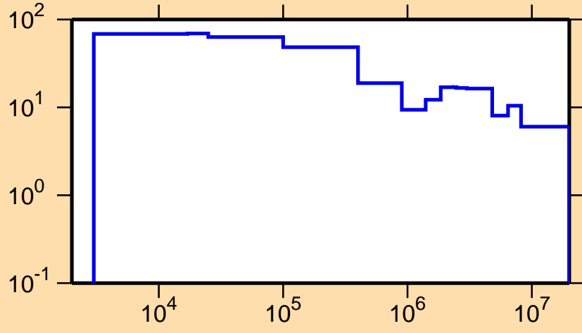
\Delta\sigma/\sigma vs. E for ^{155}\text{Sm}(n,\text{el.})
