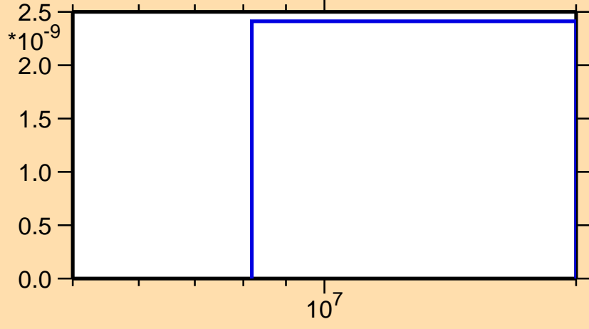
\sigma vs. E for ^{155}\text{Sm}(n,2n\alpha)
