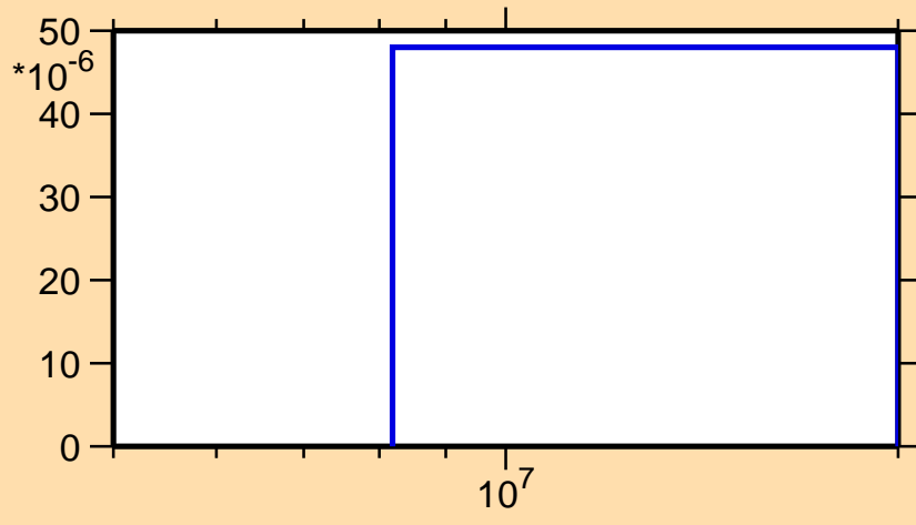
\sigma vs. E for ^{155}\text{Sm}(n,np)
