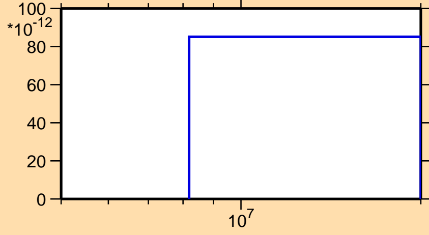
\sigma vs. E for ^{155}\text{Sm}(n,nt)
