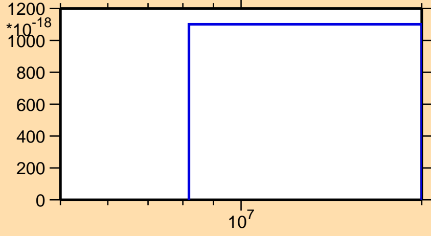
\sigma vs. E for ^{155}\text{Sm}(n,\text{He}3)
