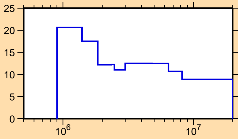
\Delta\sigma/\sigma vs. E for ^{155}\text{Sm}(n,\text{nonel.})
