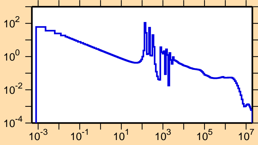
\sigma vs. E for ^{156}\text{Sm}(n,\gamma)
