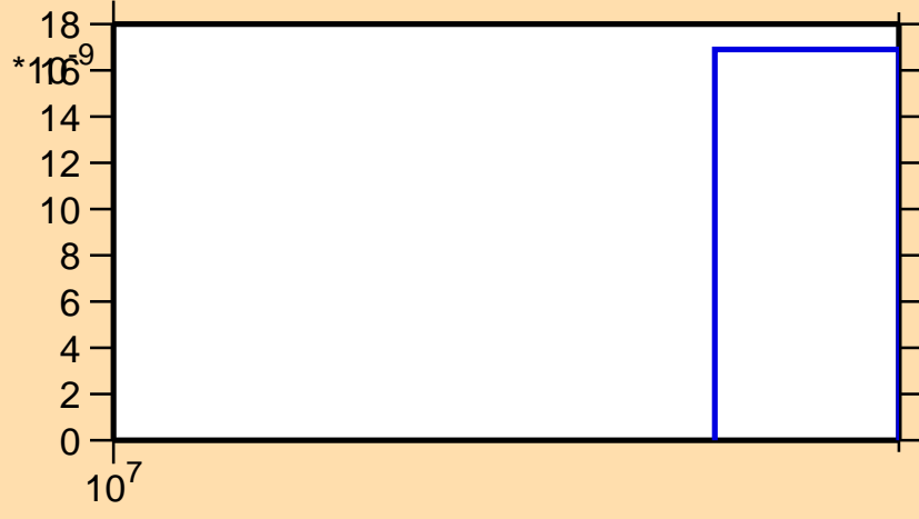
\sigma vs. E for ^{156}\text{Sm}(n,nt)
