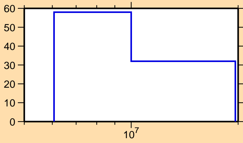
\Delta\sigma/\sigma vs. E for ^{156}\text{Sm}(n,\text{inel.})
