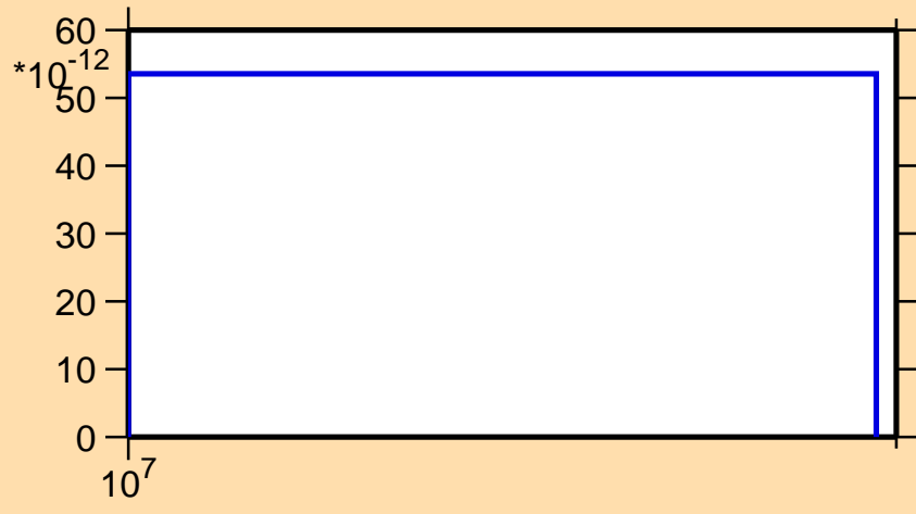
\sigma vs. E for ^{156}\text{Sm}(n,2n\alpha)
