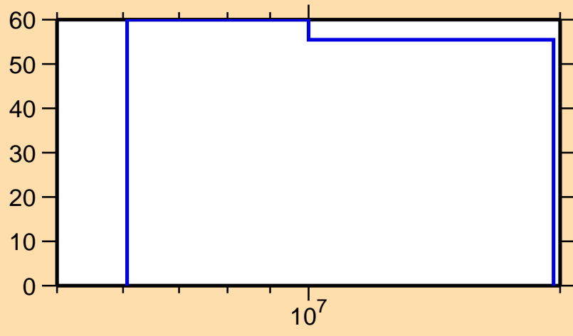
\Delta\sigma/\sigma vs. E for ^{156}\text{Sm}(n,n_1)
