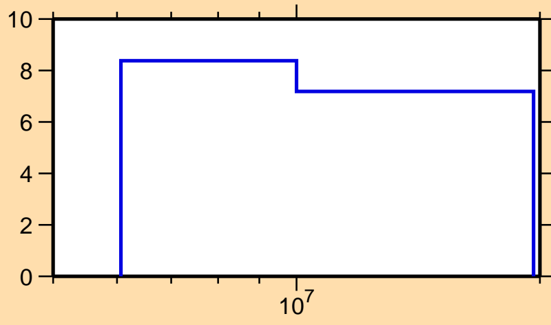
\Delta\sigma/\sigma vs. E for ^{156}\text{Sm}(n,\text{tot.})
