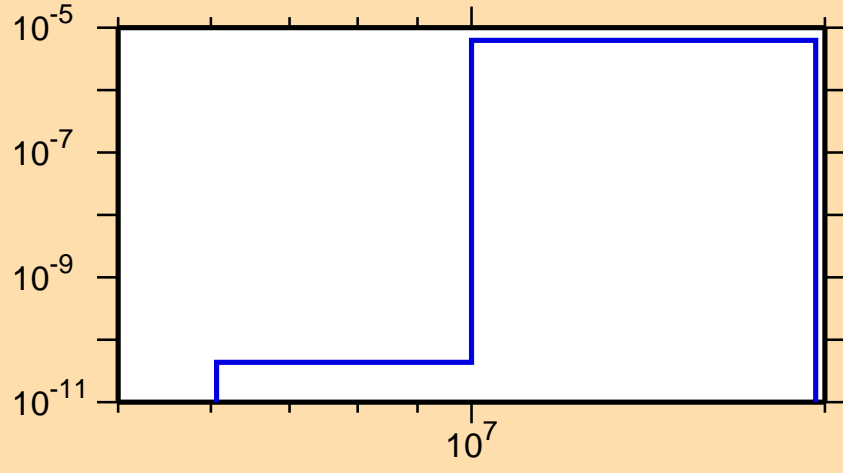
\sigma vs. E for ^{156}\text{Sm}(n,n\alpha)
