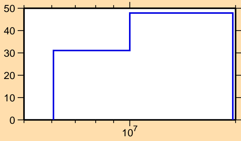
\Delta\sigma/\sigma vs. E for ^{156}\text{Sm}(n,2n)
