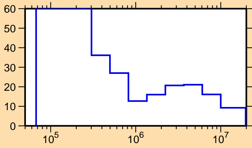
\Delta\sigma/\sigma vs. E for ^{156}\text{Sm}(n,\text{el.})
