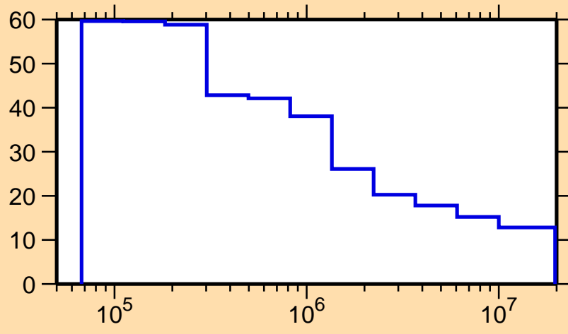
\Delta\sigma/\sigma vs. E for ^{156}\text{Sm}(n,\text{nonel.})
