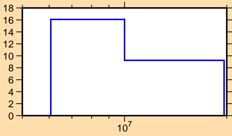
\Delta\sigma/\sigma vs. E for ^{156}\text{Sm}(n,el.)
