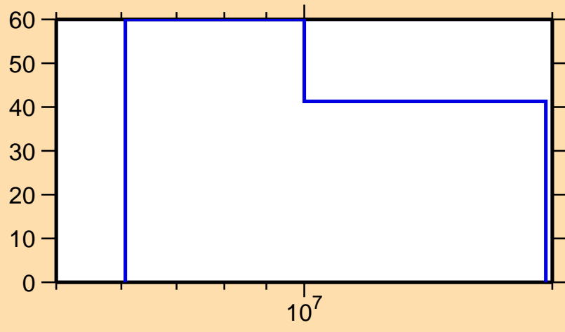
\Delta\sigma/\sigma vs. E for ^{156}\text{Sm}(n,ncont.)
