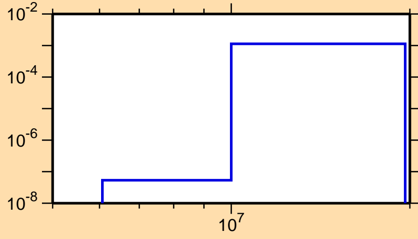
\sigma vs. E for ^{156}\text{Sm}(n,p)
