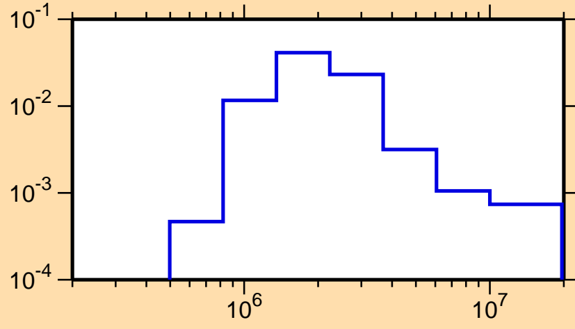
\sigma vs. E for ^{156}\text{Sm}(n,n_3)
