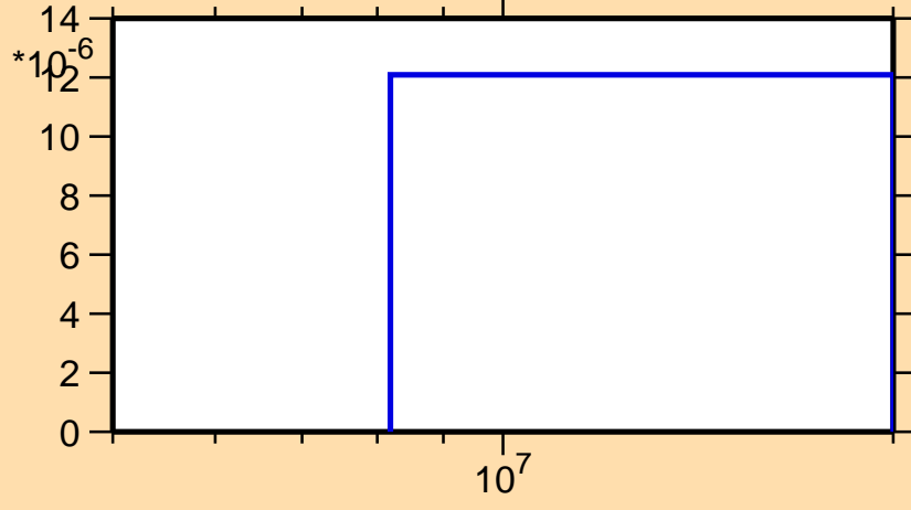
\sigma vs. E for ^{156}\text{Sm}(n,np)
