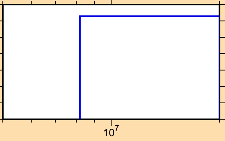
\sigma vs. E for ^{156}\text{Sm}(n,t)
