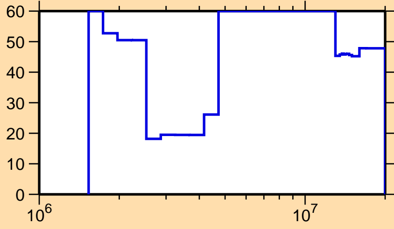
\Delta\sigma/\sigma vs. E for ^{157}\text{Sm}(n,n\text{cont.})
