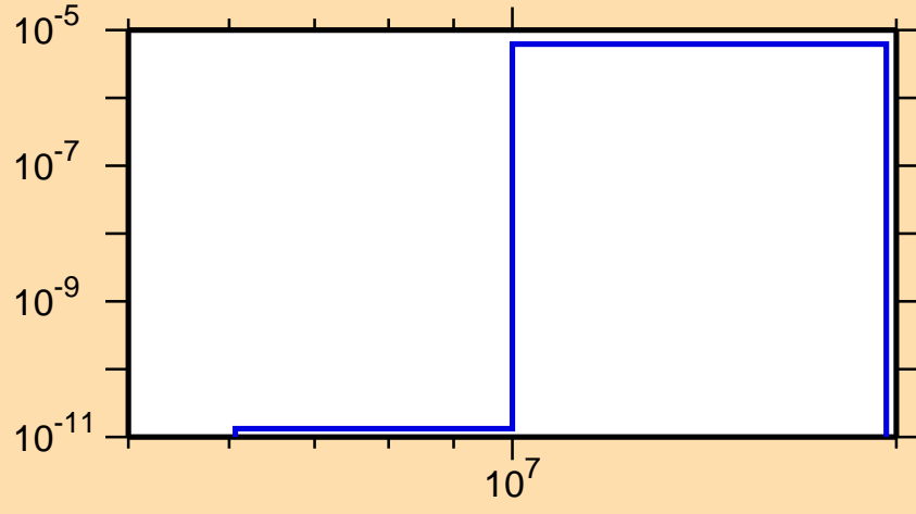
\sigma vs. E for ^{157}\text{Sm}(n,n\alpha)
