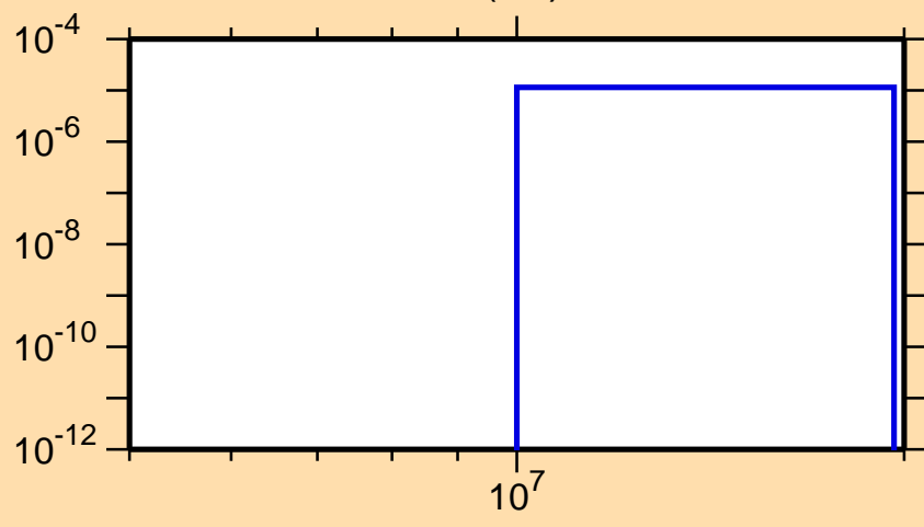
\sigma vs. E for ^{157}\text{Sm}(n,t)
