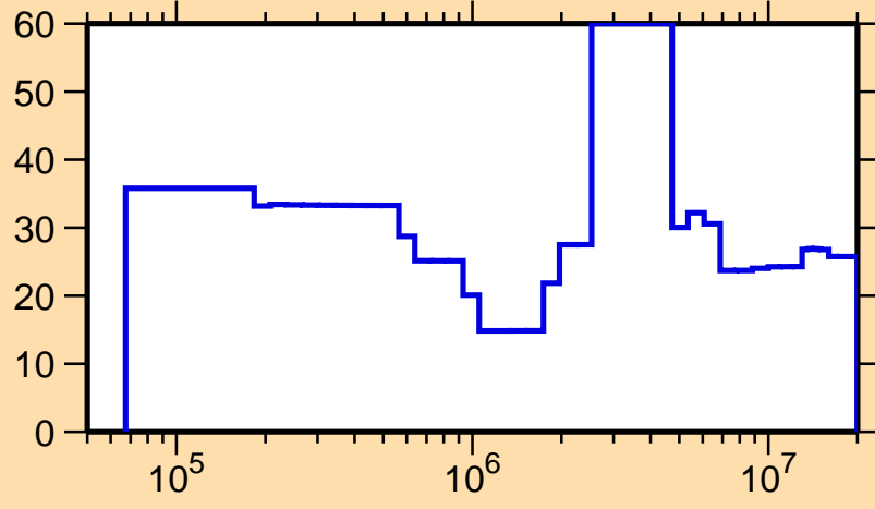
\Delta\sigma/\sigma vs. E for ^{158}\text{Sm}(n,n_1)
