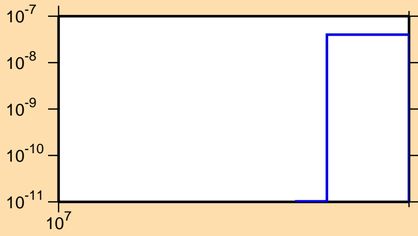
\sigma vs. E for ^{158}\text{Sm}(n,nt)
