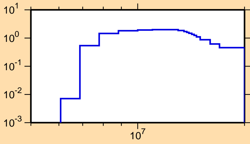
\sigma vs. E for ^{158}\text{Sm}(n,2n)
