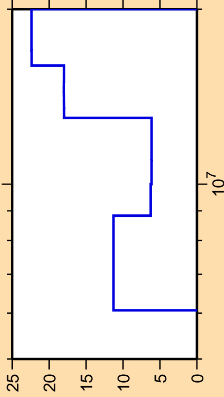
\Delta\sigma/\sigma vs. E for ^{158}\text{Sm}(n,2n)
