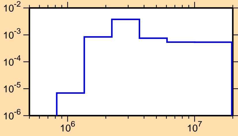
\sigma vs. E for ^{158}\text{Sm}(n,n_4)
