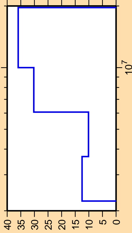
\Delta\sigma/\sigma vs. E for ^{158}\text{Sm}(n,n\text{cont.})
