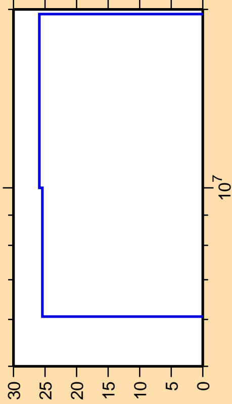
\Delta\sigma/\sigma vs. E for ^{158}\text{Sm}(n,n_1)
