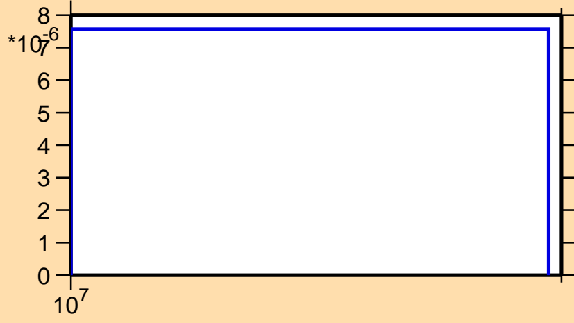
\sigma vs. E for ^{158}\text{Sm}(n,np)
