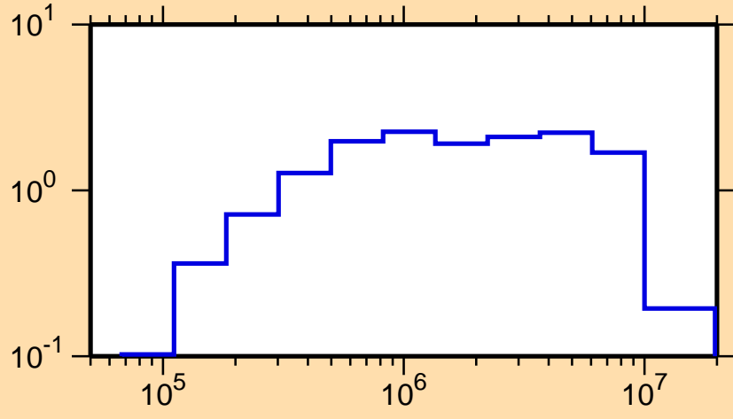
\sigma vs. E for ^{158}\text{Sm}(n,\text{inel.})
