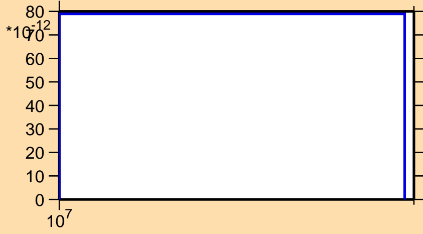
\sigma vs. E for ^{158}\text{Sm}(n,\text{nd})
