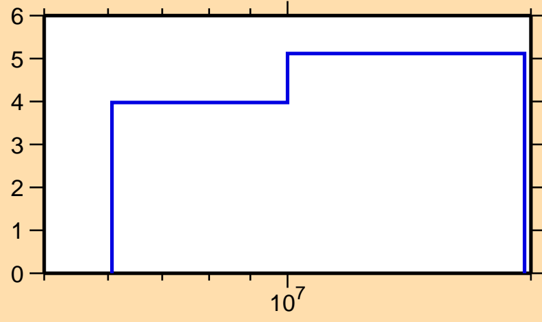
\Delta\sigma/\sigma vs. E for ^{158}\text{Sm}(n,\text{el.})
