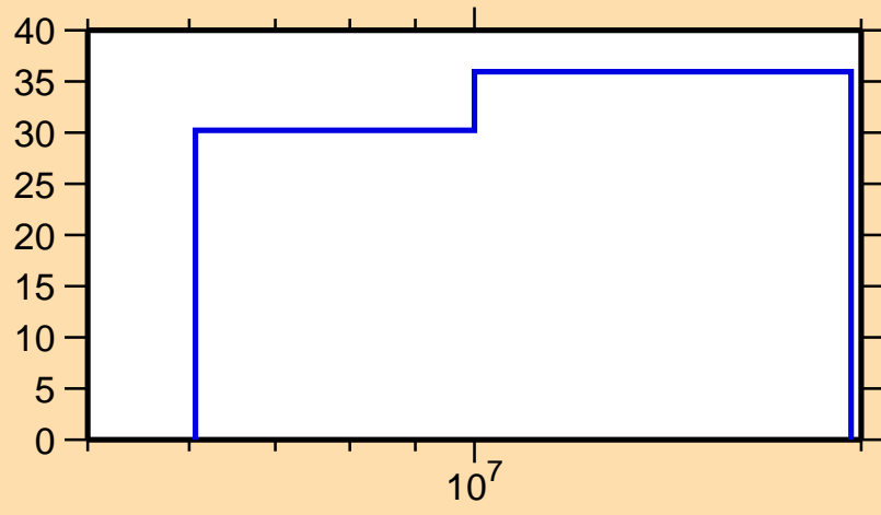
\Delta\sigma/\sigma vs. E for ^{158}\text{Sm}(n,n\text{cont.})
