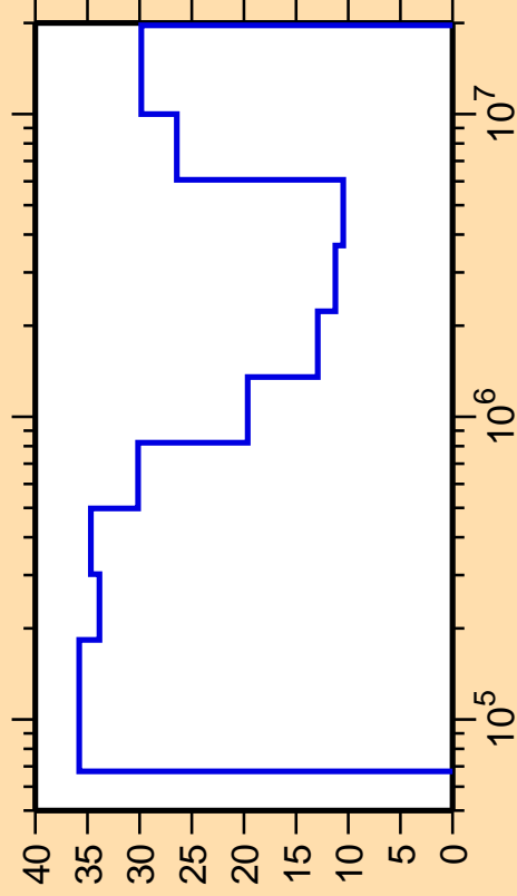
\Delta\sigma/\sigma vs. E for ^{158}\text{Sm}(n,\text{inel.})
