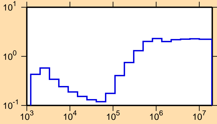
\sigma vs. E for ^{158}\text{Sm}(n,\text{nonel.})
