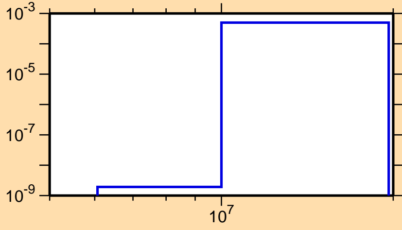
\sigma vs. E for ^{158}\text{Sm}(n,p)
