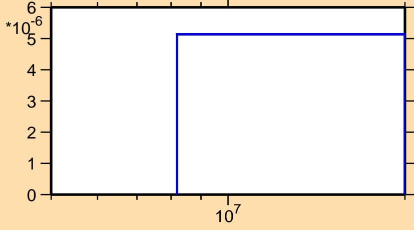
\sigma vs. E for ^{158}\text{Sm}(n,t)
