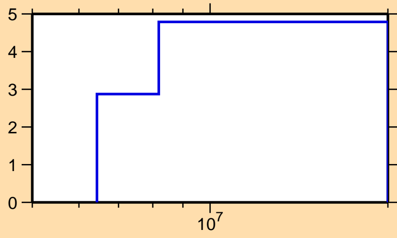
\Delta\sigma/\sigma vs. E for ^{158}\text{Sm}(n,el.)
