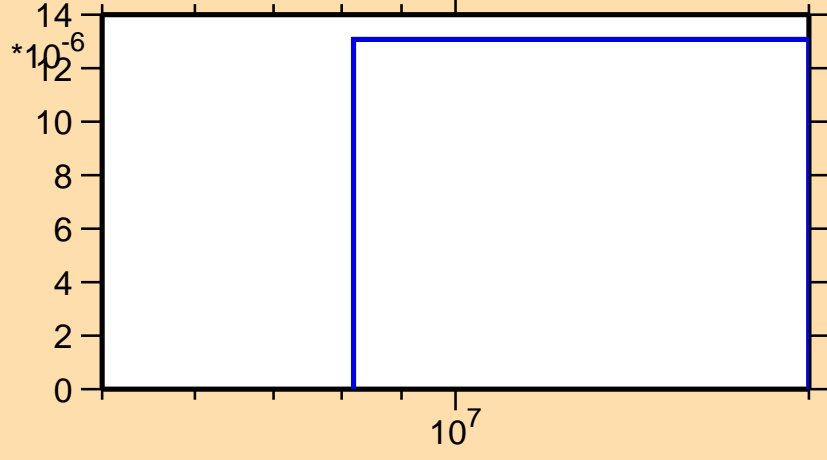
\sigma vs. E for ^{158}\text{Sm}(n,d)
