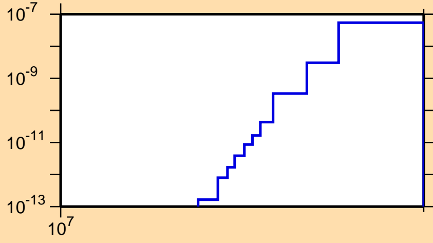
\sigma vs. E for ^{159}\text{Sm}(n,2n\alpha)
