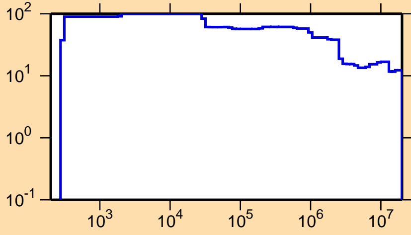
\Delta\sigma/\sigma vs. E for ^{159}\text{Sm}(n,\text{nonel.})
