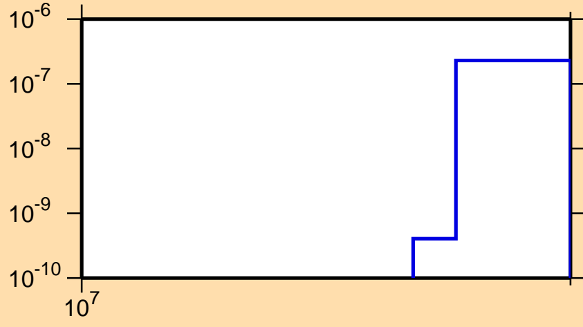
\sigma vs. E for ^{159}\text{Sm}(n,\text{nd})
