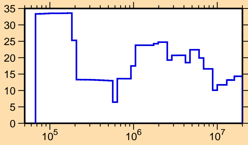
\Delta\sigma/\sigma vs. E for ^{159}\text{Sm}(n,\text{el.})
