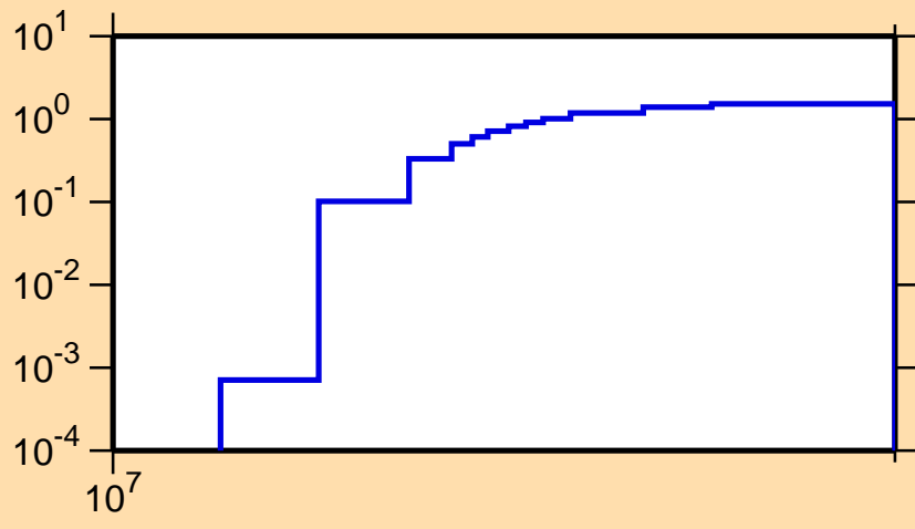
\sigma vs. E for ^{159}\text{Sm}(n,3n)
