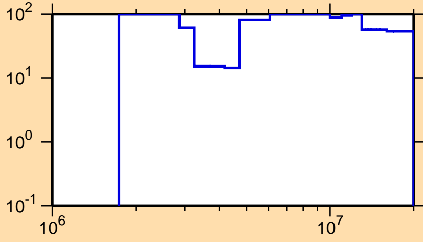
\Delta\sigma/\sigma vs. E for ^{159}\text{Sm}(n,n\text{cont.})
