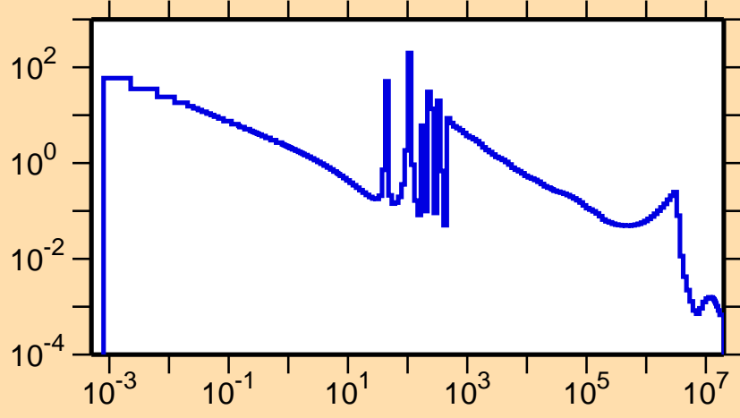
\sigma vs. E for ^{159}\text{Sm}(n,\gamma)
