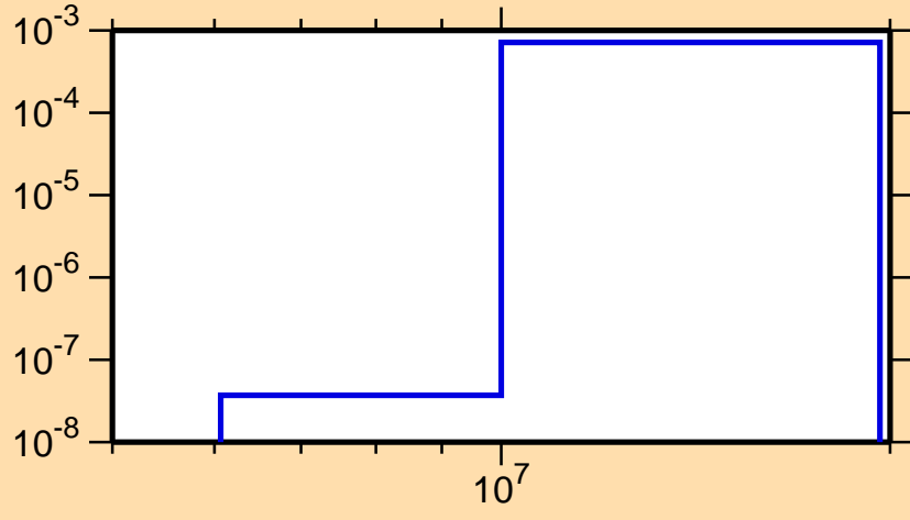
\sigma vs. E for ^{159}\text{Sm}(n,p)
