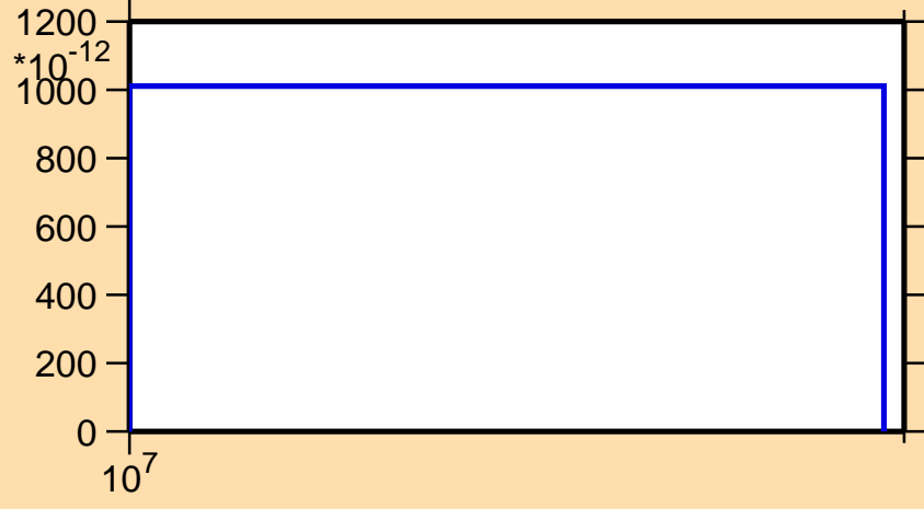
\sigma vs. E for ^{159}\text{Sm}(n,nt)
