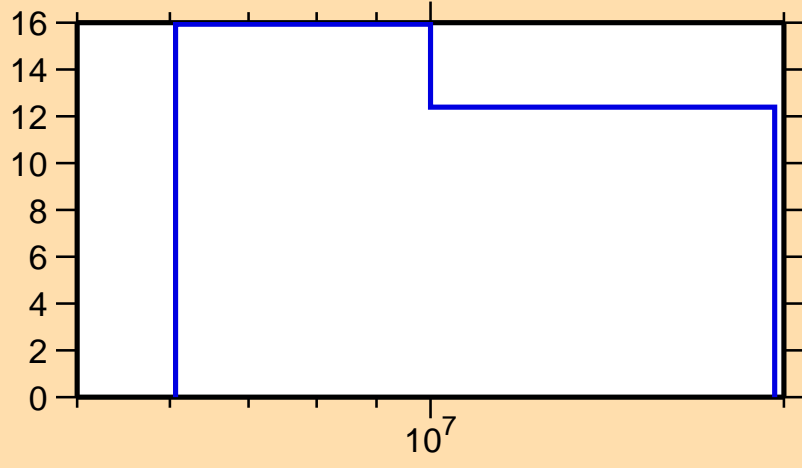
\Delta\sigma/\sigma vs. E for ^{159}\text{Sm}(n,el.)
