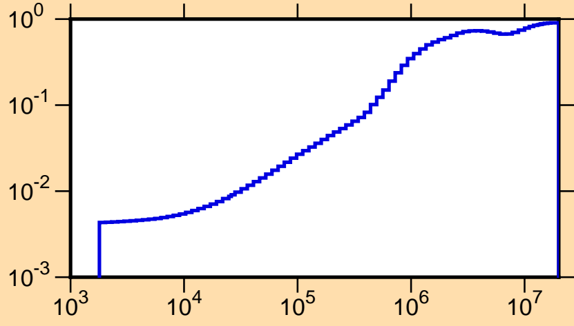
\mu vs. E for ^{160}\text{Sm}(\text{mt251})
