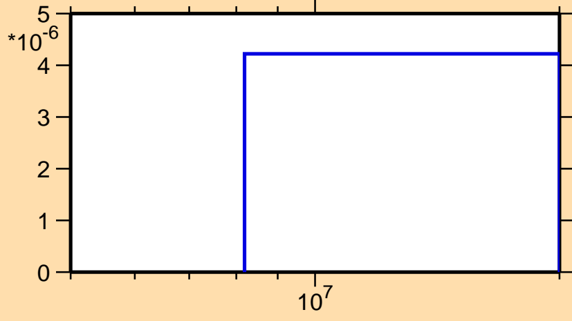
\sigma vs. E for ^{160}\text{Sm}(n,t)
