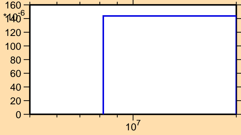
\sigma vs. E for ^{160}\text{Sm}(n,p)
