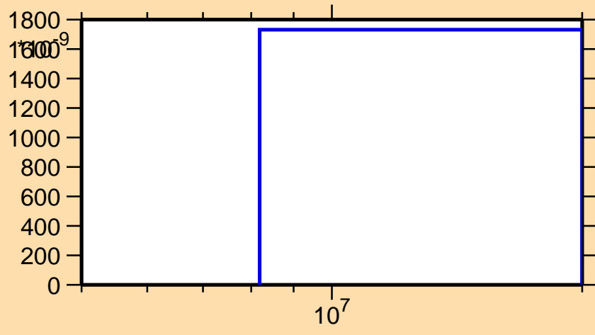
\sigma vs. E for ^{160}\text{Sm}(n,np)
