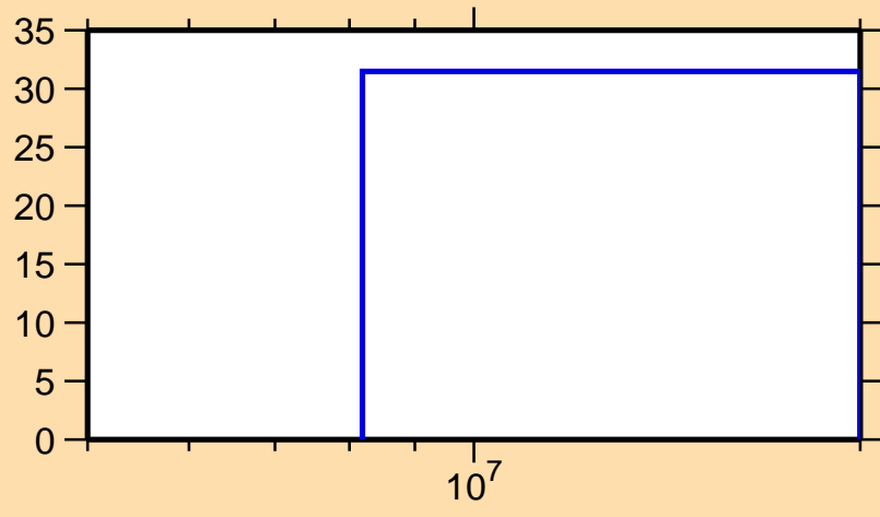
\Delta\sigma/\sigma vs. E for ^{160}\text{Sm}(n,el.)
