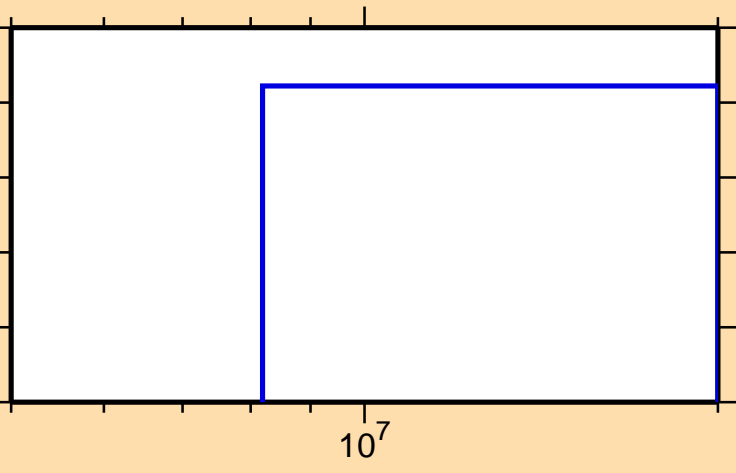
\sigma vs. E for ^{160}\text{Sm}(n,t)
