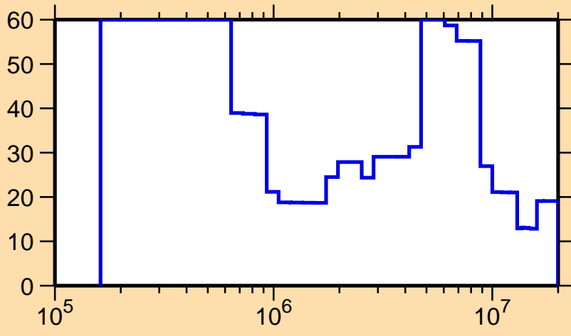
\Delta\sigma/\sigma vs. E for ^{161}\text{Sm}(n,\text{el.})
