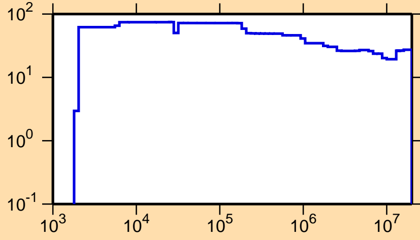
\Delta\sigma/\sigma vs. E for ^{161}\text{Sm}(n,\text{nonel.})
