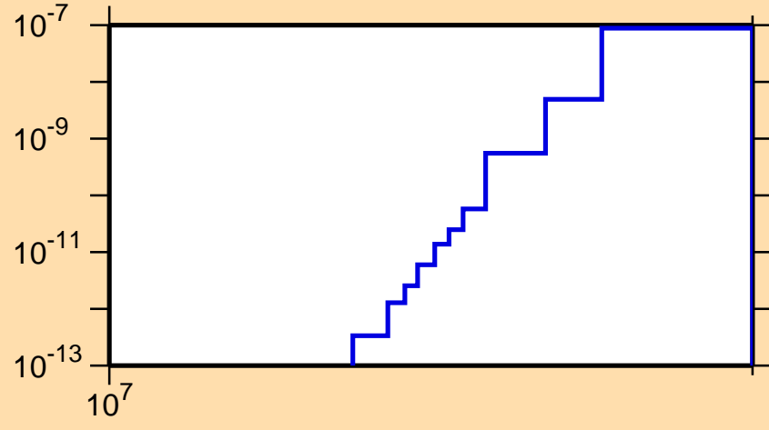
\sigma vs. E for ^{161}\text{Sm}(n,2n\alpha)
