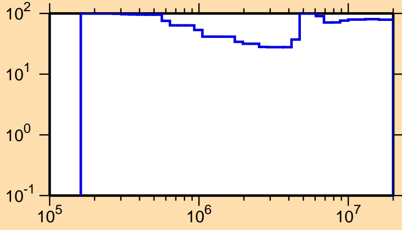
\Delta\sigma/\sigma vs. E for ^{161}\text{Sm}(n,n\text{cont.})
