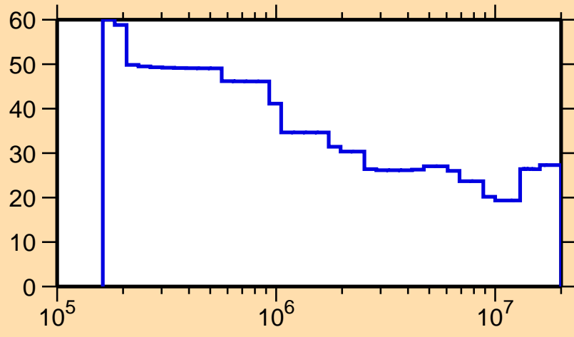
\Delta\sigma/\sigma vs. E for ^{161}\text{Sm}(n,\text{nonel.})
