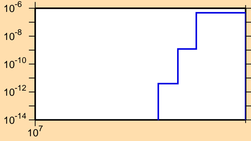
\sigma vs. E for ^{161}\text{Sm}(n,nt)
