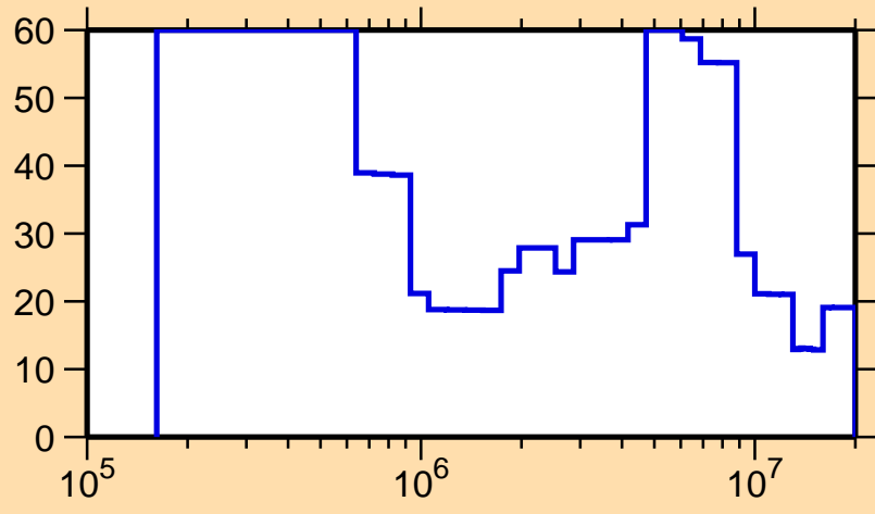
\Delta\sigma/\sigma vs. E for ^{161}\text{Sm}(n, el.)
