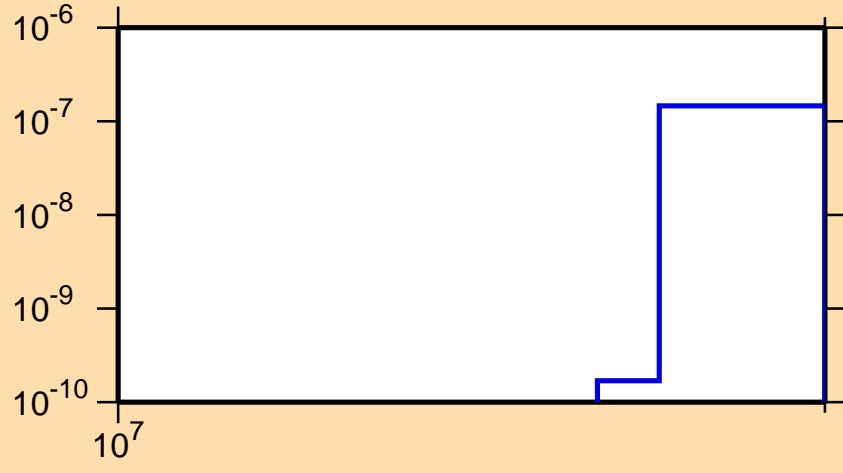
\sigma vs. E for ^{161}\text{Sm}(n,\text{nd})
