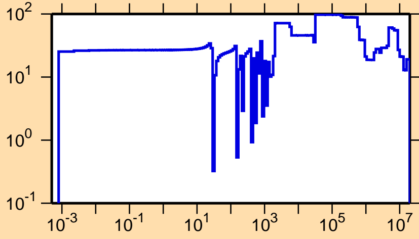
\Delta\sigma/\sigma vs. E for ^{161}\text{Sm}(n,\text{el.})
