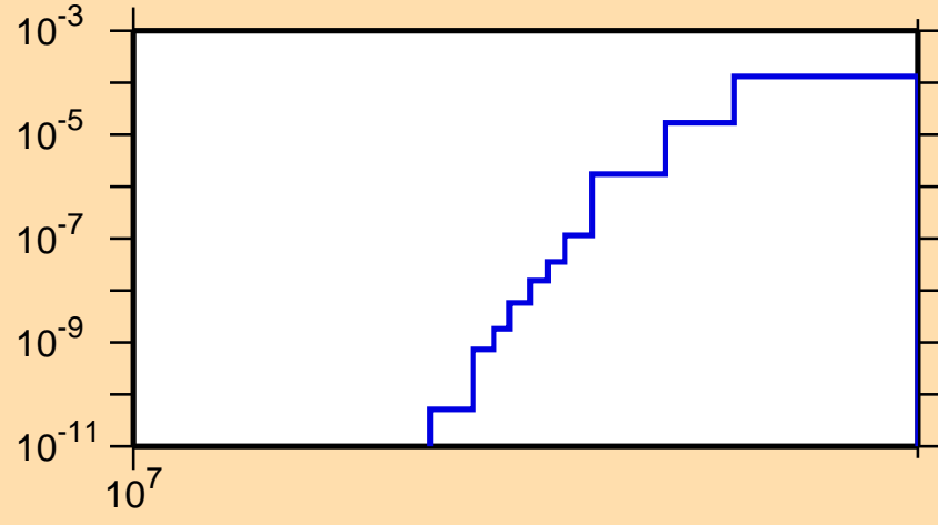
\sigma vs. E for ^{161}\text{Sm}(n,np)
