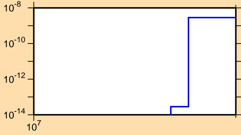
\sigma vs. E for ^{161}\text{Sm}(n,2np)
