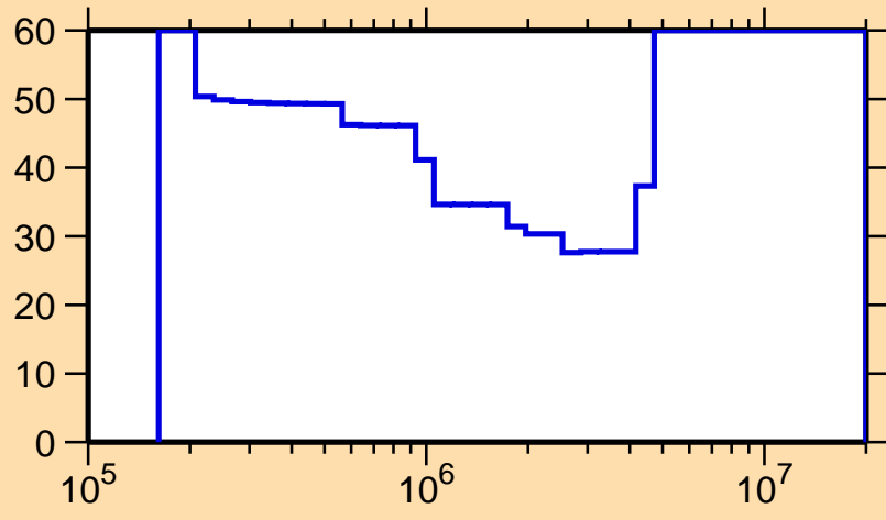
\Delta\sigma/\sigma vs. E for ^{161}\text{Sm}(n,\text{inel.})
