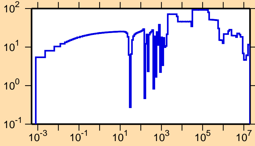
\Delta\sigma/\sigma vs. E for ^{161}\text{Sm}(n,\text{tot.})
