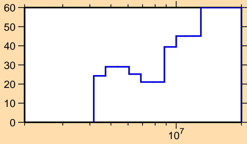
\Delta\sigma/\sigma vs. E for ^{161}\text{Sm}(n,2n)
