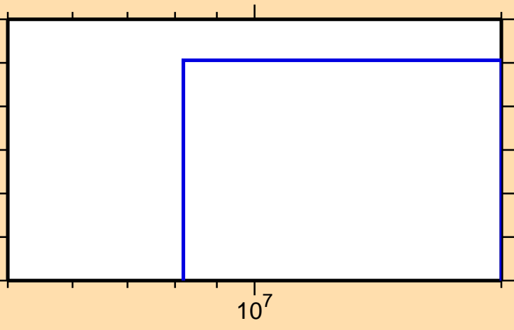
\sigma vs. E for ^{161}\text{Sm}(n,t)
