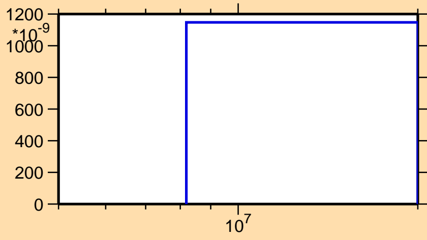
\sigma vs. E for ^{161}\text{Sm}(n,\alpha)
