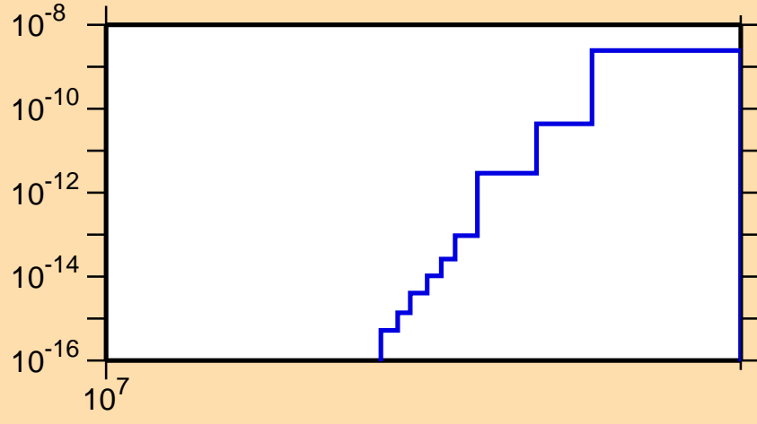
\sigma vs. E for ^{162}\text{Sm}(n,2n\alpha)
