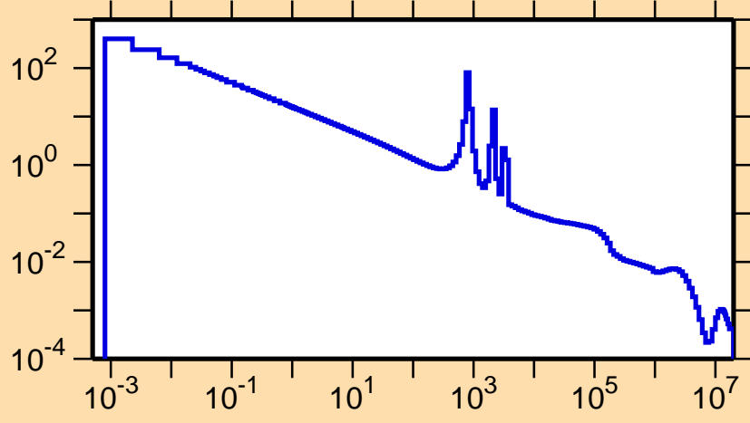
\sigma vs. E for ^{162}\text{Sm}(n,\gamma)
