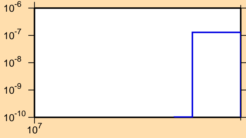
\sigma vs. E for ^{162}\text{Sm}(n,nt)
