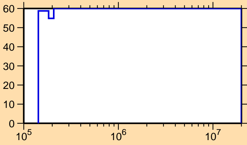
\Delta\sigma/\sigma vs. E for ^{162}\text{Sm}(n,n_1)
