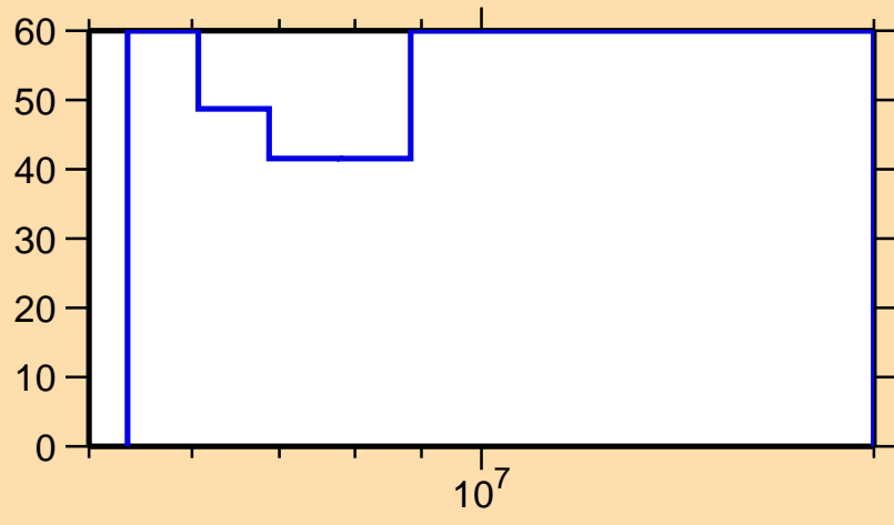
\Delta\sigma/\sigma vs. E for ^{162}\text{Sm}(n,2n)
