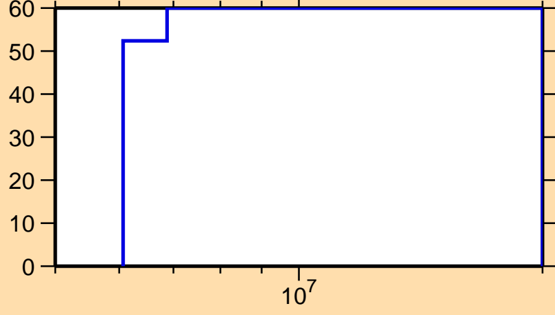
\Delta\sigma/\sigma vs. E for ^{162}\text{Sm}(n,n\text{cont.})
