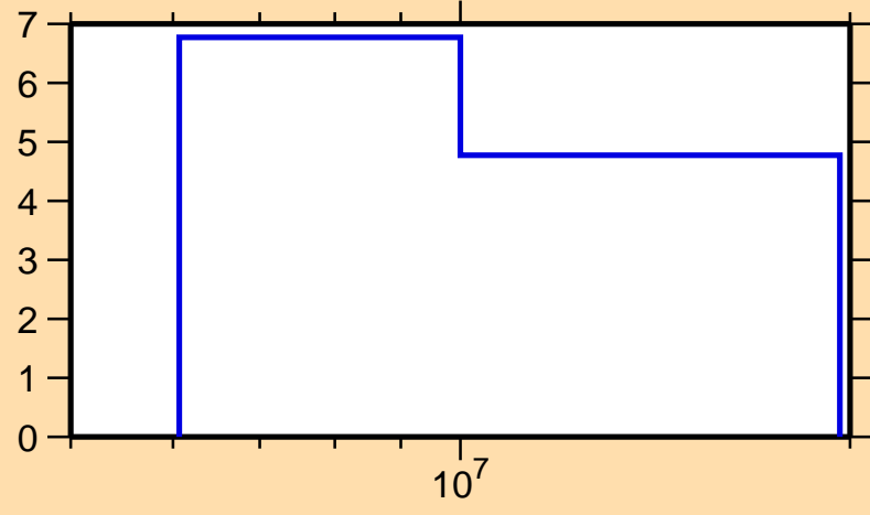
\Delta\sigma/\sigma vs. E for ^{163}\text{Sm}(n,\text{tot.})
