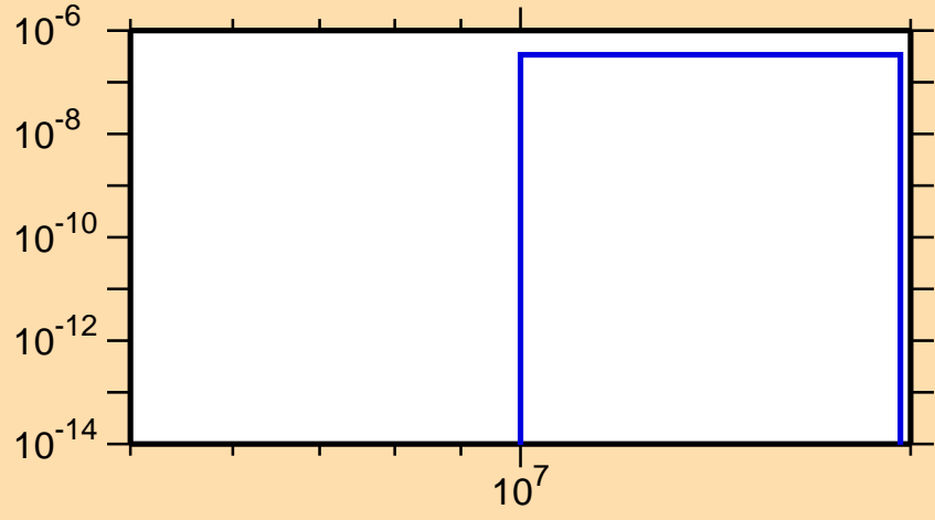
\sigma vs. E for ^{163}\text{Sm}(n,n\alpha)
