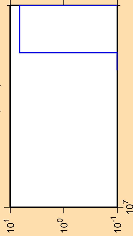
\Delta\sigma/\sigma vs. E for ^{100}\text{Sn}(n,\text{nd})
