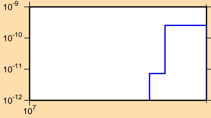
\sigma vs. E for ^{100}\text{Sn}(\text{mt117})
