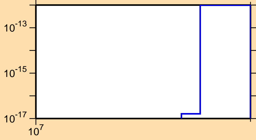
\sigma vs. E for ^{100}\text{Sn}(n,\text{nd})
