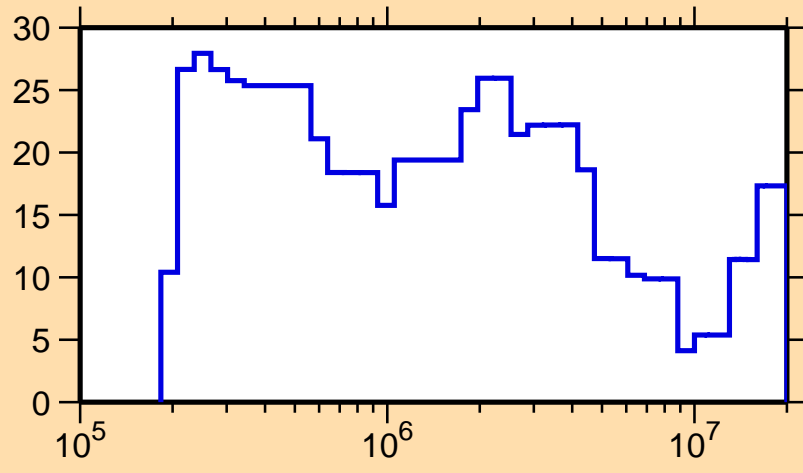
\Delta\sigma/\sigma vs. E for ^{100}\text{Sn}(n,el.)
