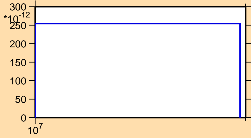
\sigma vs. E for ^{100}\text{Sn} (mt 45)
