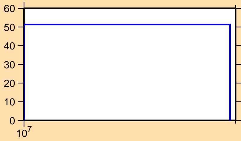
\Delta\sigma/\sigma vs. E for ^{100}\text{Sn}(n,2n)
