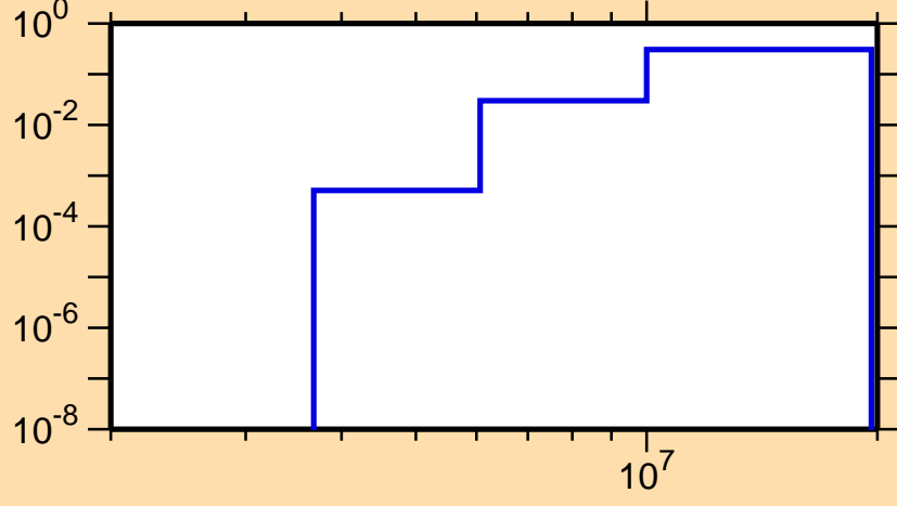
\sigma vs. E for ^{100}\text{Sn}(n,np)
