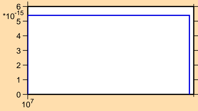
\sigma vs. E for ^{100}\text{Sn}(n,\text{nd})
