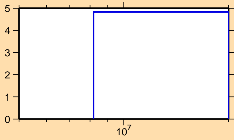
\Delta\sigma/\sigma vs. E for ^{100}\text{Sn}(n,\text{nonel.})
