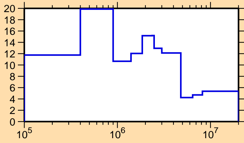
\Delta\sigma/\sigma vs. E for ^{100}\text{Sn}(n,\text{tot.})
