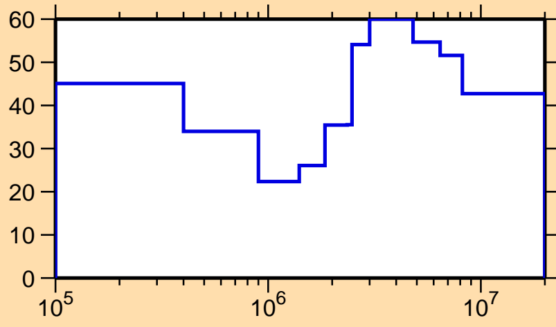
\Delta\sigma/\sigma vs. E for ^{100}\text{Sn}(n,n_1)
