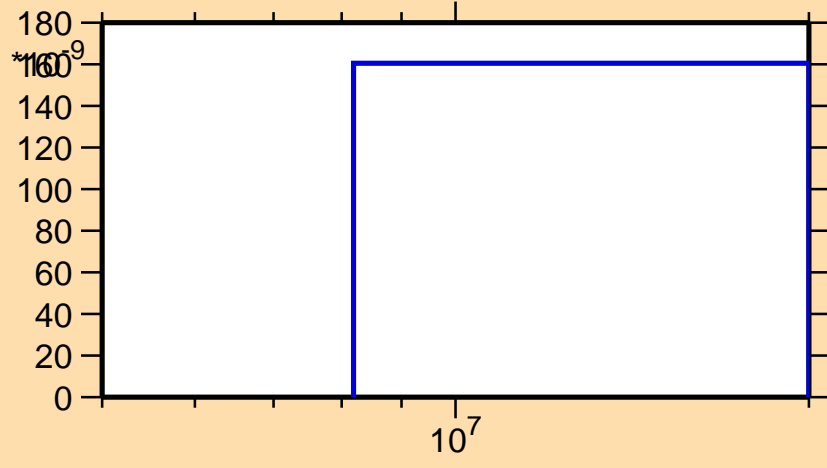
\sigma vs. E for ^{100}\text{Sn}(n,2n)
