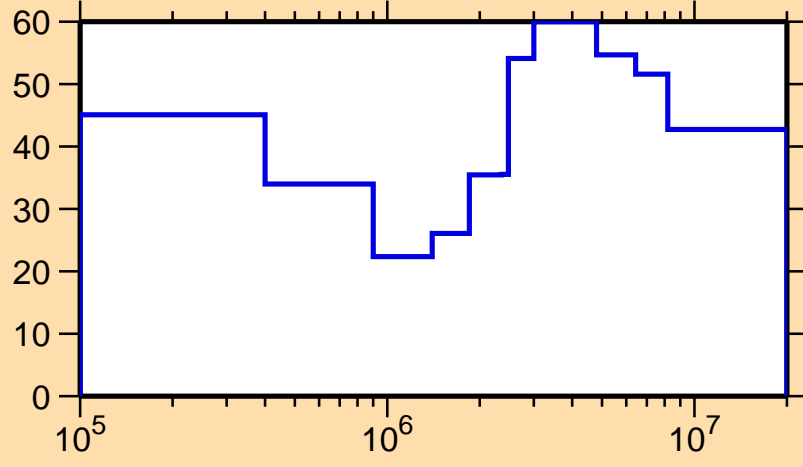
\Delta\sigma/\sigma vs. E for ^{100}\text{Sn}(n,n_1)
