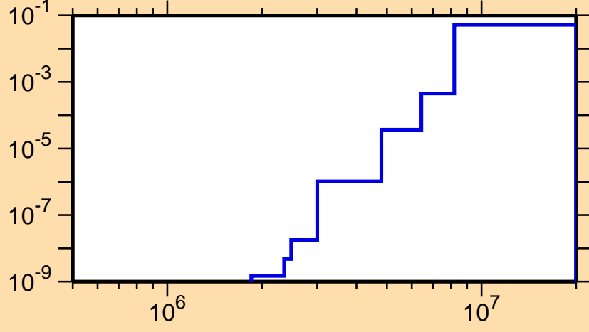
\sigma vs. E for ^{100}\text{Sn}(n,p\alpha)
