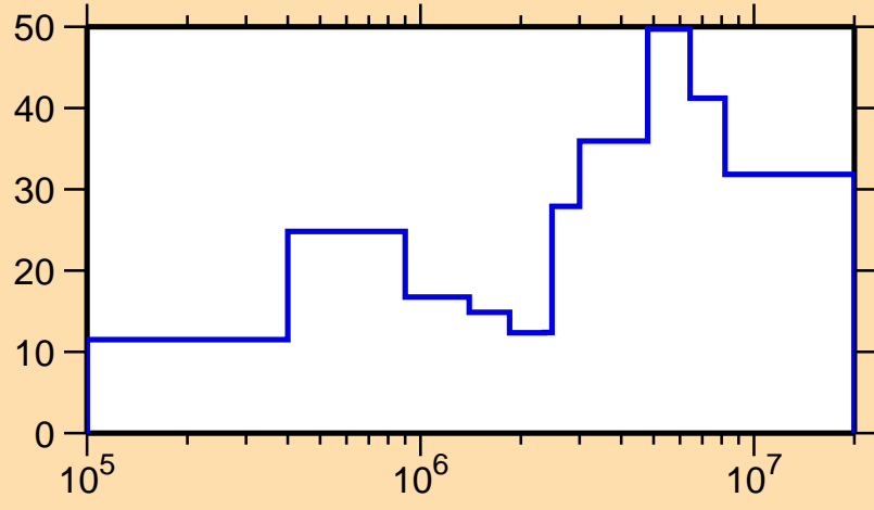
\Delta\sigma/\sigma vs. E for ^{100}\text{Sn}(n,p)
