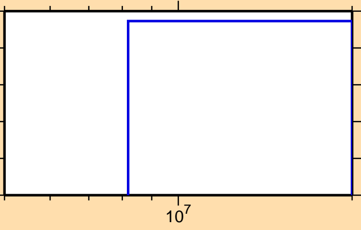
\sigma vs. E for ^{100}\text{Sn}(n,n\alpha)
