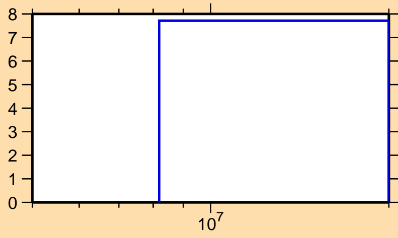
\Delta\sigma/\sigma vs. E for ^{100}\text{Sn}(n,\text{el.})
