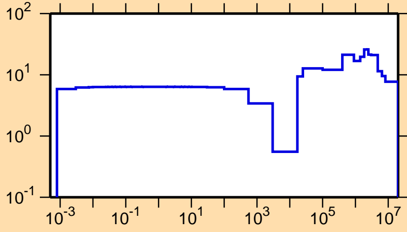
\Delta\sigma/\sigma vs. E for ^{100}\text{Sn}(n,\text{el.})
