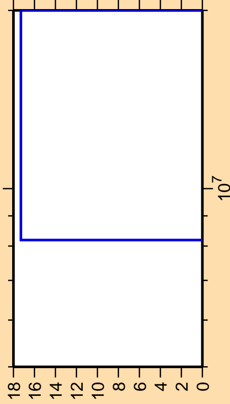
\Delta\sigma/\sigma vs. E for ^{100}\text{Sn}(\text{mt117})
