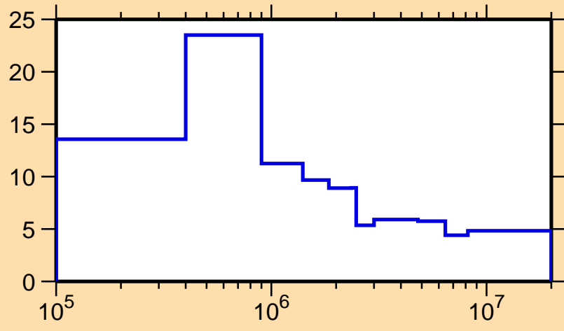
\Delta\sigma/\sigma vs. E for ^{100}\text{Sn}(n,\text{nonel.})
