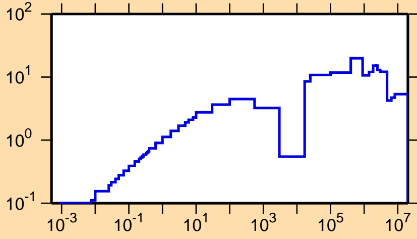
\Delta\sigma/\sigma vs. E for ^{100}\text{Sn}(n,\text{tot.})
