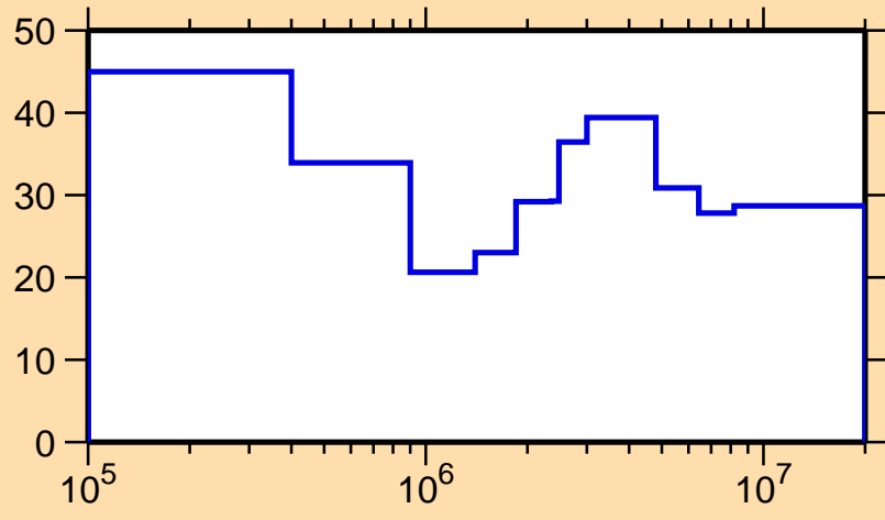
\Delta\sigma/\sigma vs. E for ^{100}\text{Sn}(n,\text{inel.})
