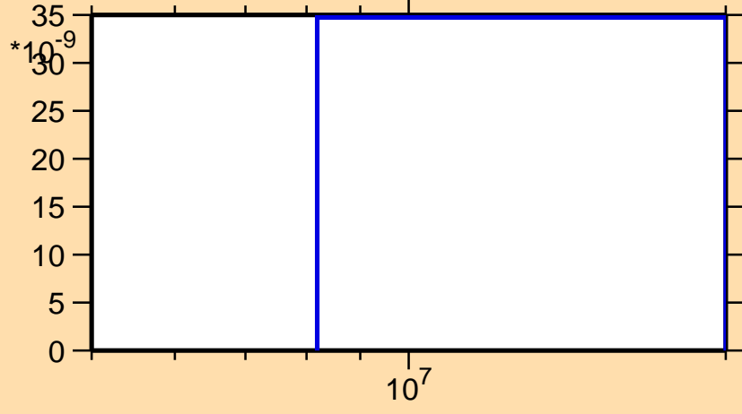
\sigma vs. E for ^{100}\text{Sn}(n,\text{pt})
