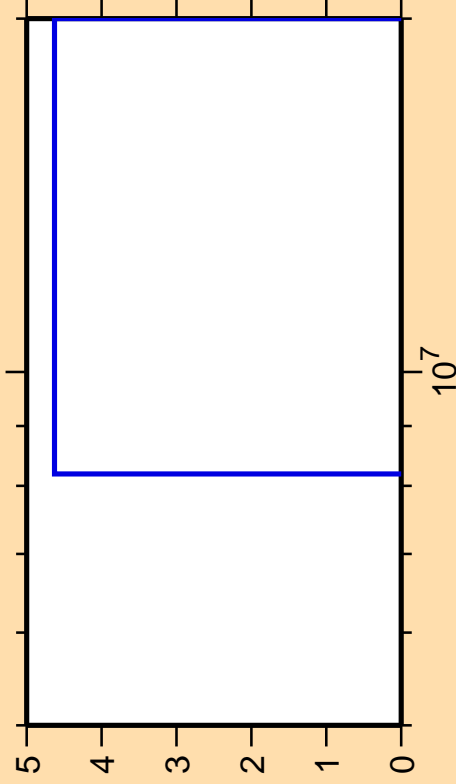
\Delta\sigma/\sigma vs. E for ^{100}\text{Sn}(\text{mt } 34)
