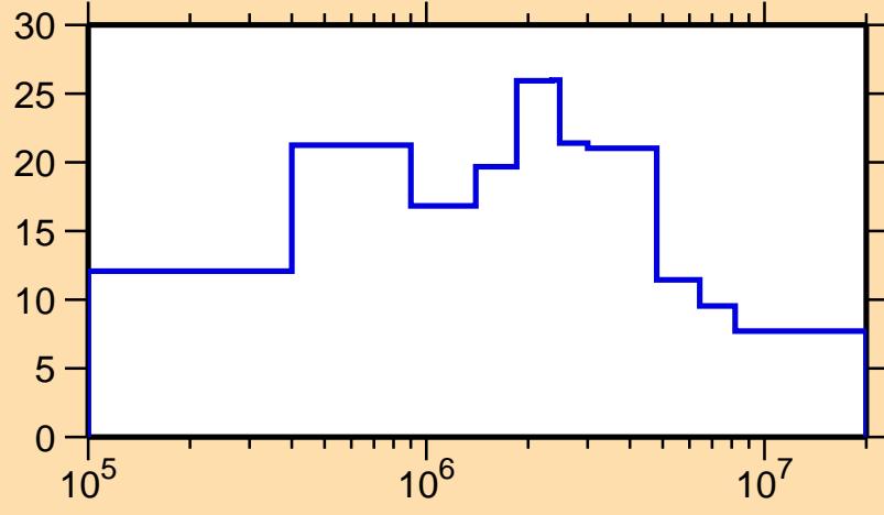
\Delta\sigma/\sigma vs. E for ^{100}\text{Sn}(n,\text{el.})
