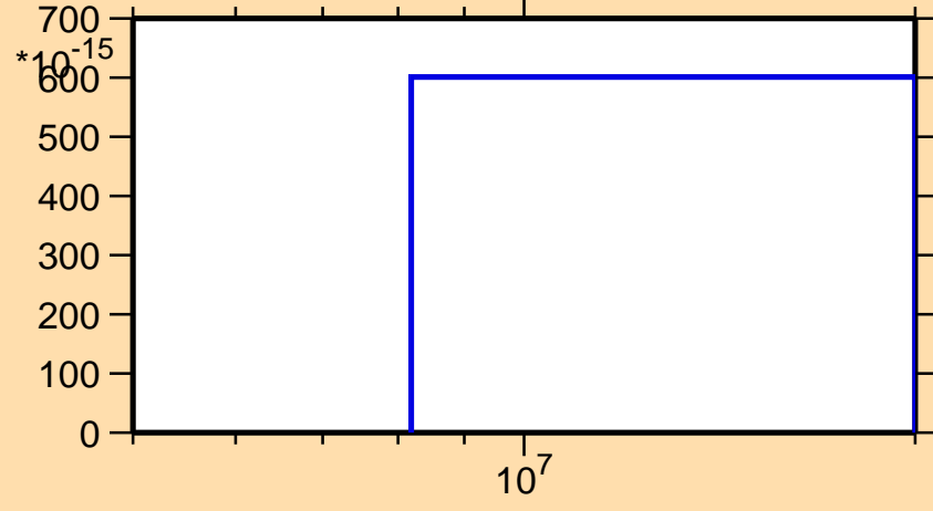
\sigma vs. E for ^{100}\text{Sn}(\text{mt } 34)
