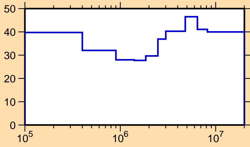
\Delta\sigma/\sigma vs. E for ^{100}\text{Sn}(n,n\text{cont.})
