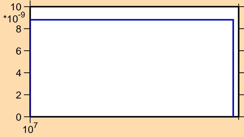
\sigma vs. E for ^{101}\text{Sn} (mt 45)
