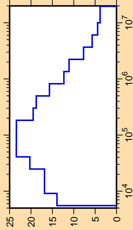
\Delta\sigma/\sigma vs. E for ^{101}\text{Sn}(n,\text{nonel.})
