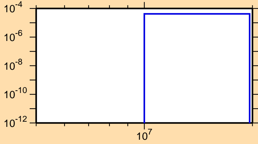
\sigma vs. E for ^{101}\text{Sn}(n,pt)
