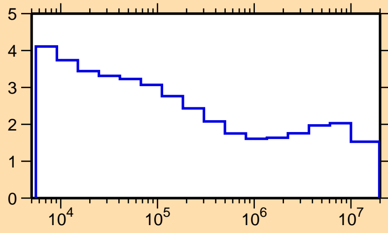
\sigma vs. E for ^{101}\text{Sn}(n,\text{nonel.})
