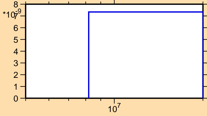
\sigma vs. E for ^{101}\text{Sn}(\text{mt } 45)
