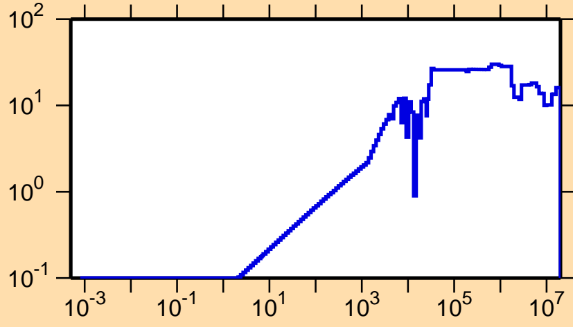
\Delta\sigma/\sigma vs. E for ^{102}\text{Sn}(n,\text{tot.})
