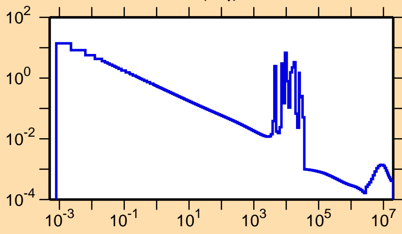
\sigma vs. E for ^{102}\text{Sn}(n,\gamma)
