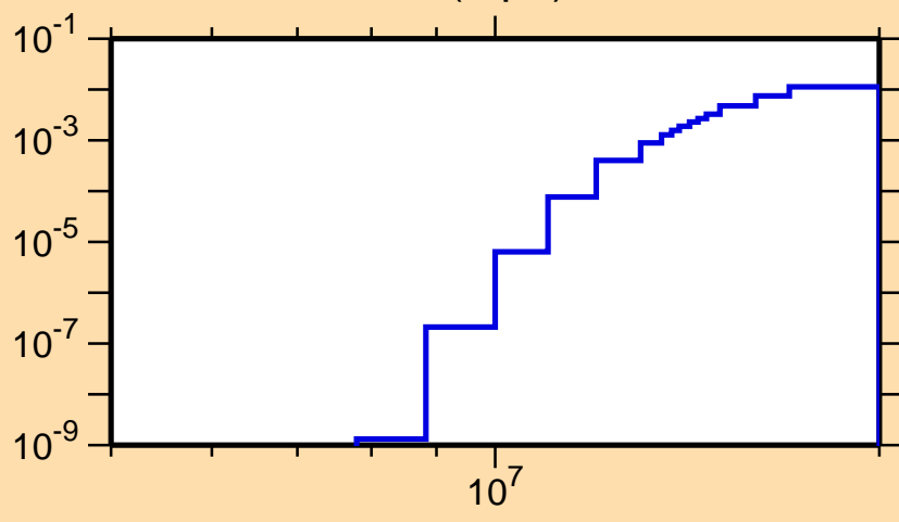
\sigma vs. E for ^{102}\text{Sn}(n,pd)
