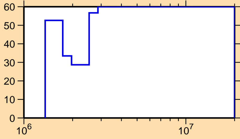
\Delta\sigma/\sigma vs. E for ^{102}\text{Sn}(n,n_1)
