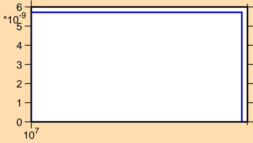
\sigma vs. E for ^{102}\text{Sn}(n,2np)
