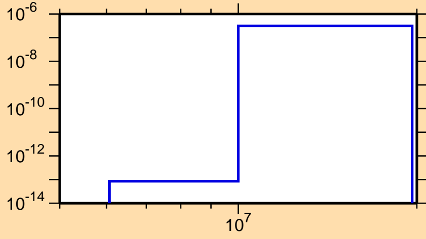
\sigma vs. E for ^{102}\text{Sn}(\text{mt117})
