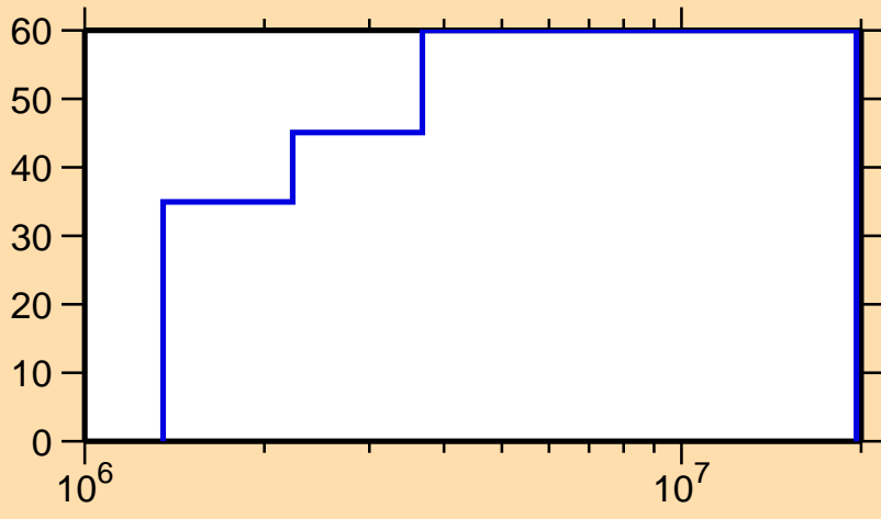
\Delta\sigma/\sigma vs. E for ^{102}\text{Sn}(n,n_1)
