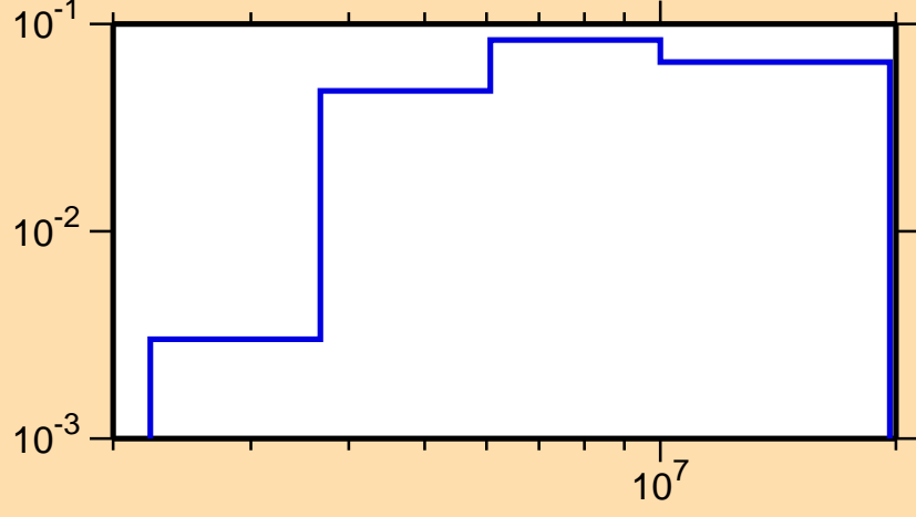
\sigma vs. E for ^{102}\text{Sn}(n,n\text{cont.})
