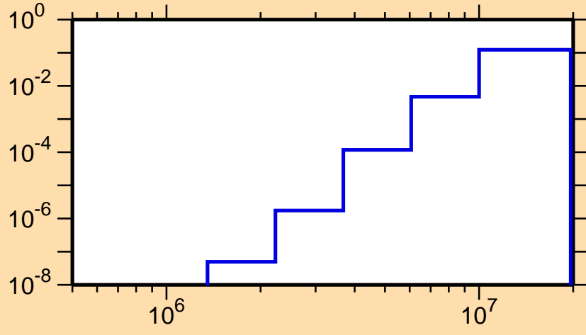
\sigma vs. E for ^{102}\text{Sn}(n,p\alpha)
