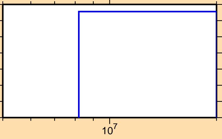
\sigma vs. E for ^{102}\text{Sn}(n,2np)
