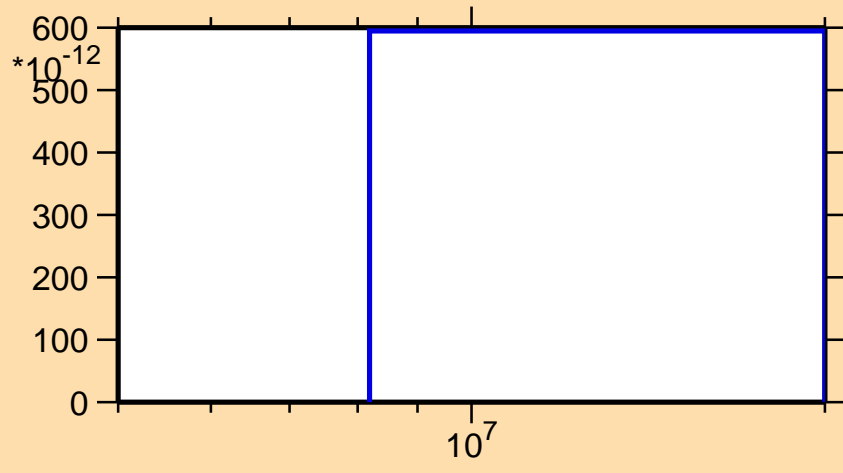
\sigma vs. E for ^{102}\text{Sn}(n,nd)
