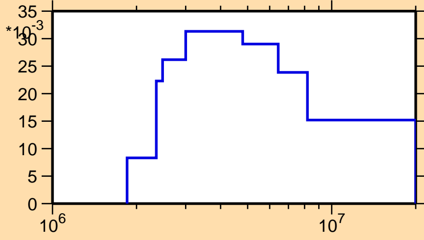
\sigma vs. E for ^{102}\text{Sn}(n,n_2)
