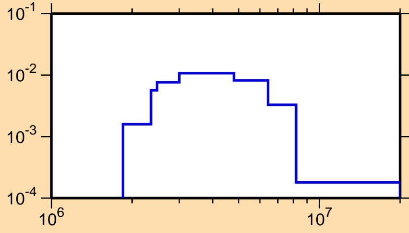
\sigma vs. E for ^{102}\text{Sn}(n,n_4)
