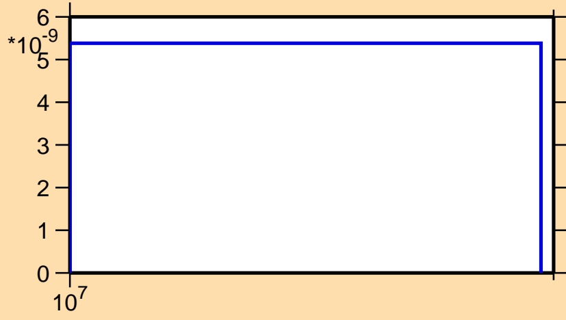
\sigma vs. E for ^{103}\text{Sn} (mt 34)
