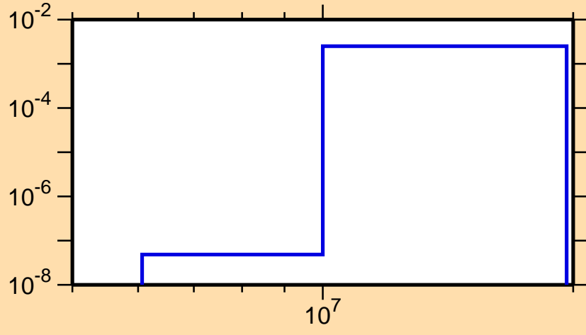
\sigma vs. E for ^{103}\text{Sn}(n,\text{pd})
