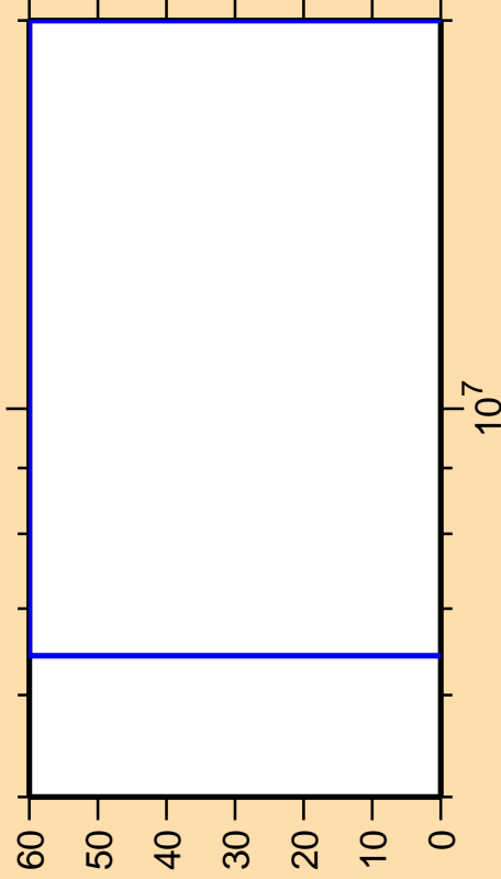
\Delta\sigma/\sigma vs. E for ^{103}\text{Sn}(n,\text{pd})
