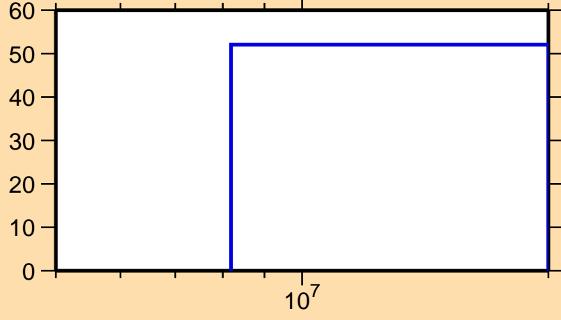
\Delta\sigma/\sigma vs. E for ^{103}\text{Sn}(n,\text{inel.})
