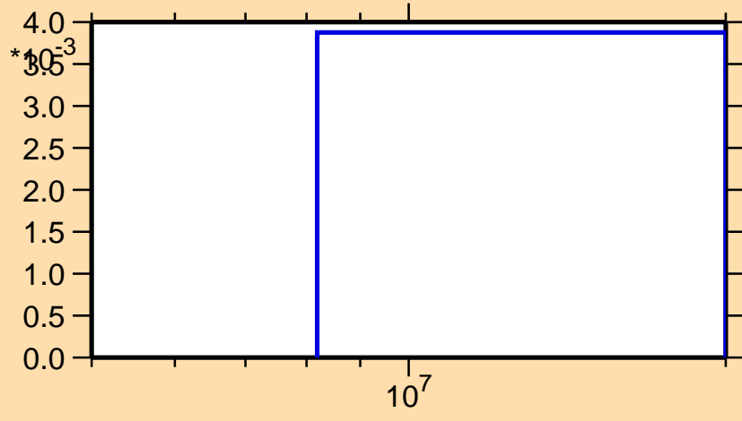
\sigma vs. E for ^{103}\text{Sn}(n,2n)
