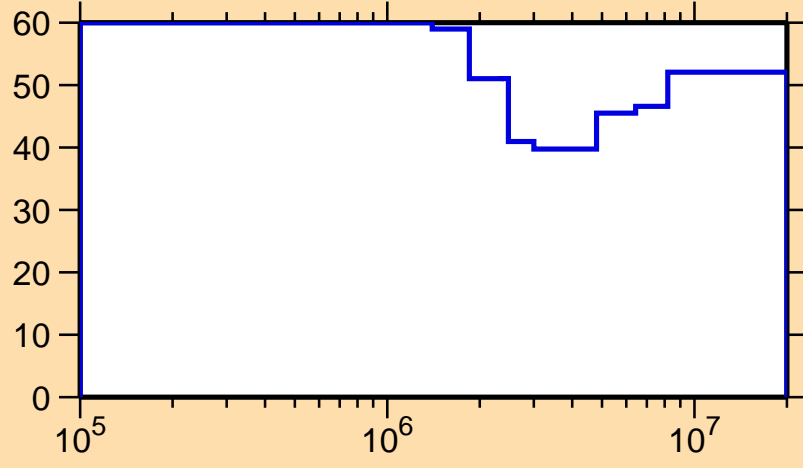
\Delta\sigma/\sigma vs. E for ^{103}\text{Sn}(n,\text{inel.})
