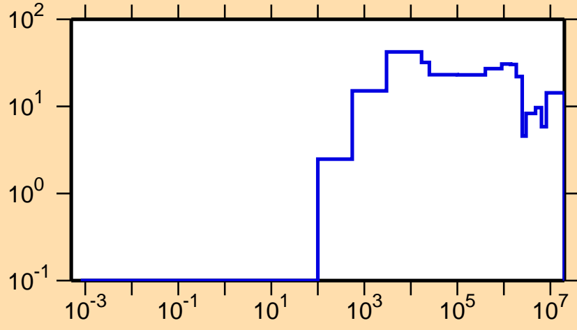
\Delta\sigma/\sigma vs. E for ^{103}\text{Sn}(n,\text{tot.})
