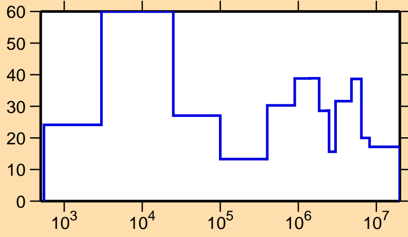
\Delta\sigma/\sigma vs. E for ^{103}\text{Sn}(n,\text{el.})
