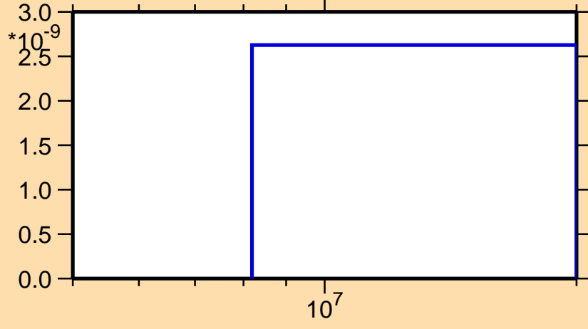
\sigma vs. E for ^{103}\text{Sn}(n,2n\alpha)
