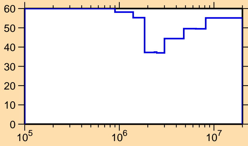
\Delta\sigma/\sigma vs. E for ^{103}\text{Sn}(n,n_1)
