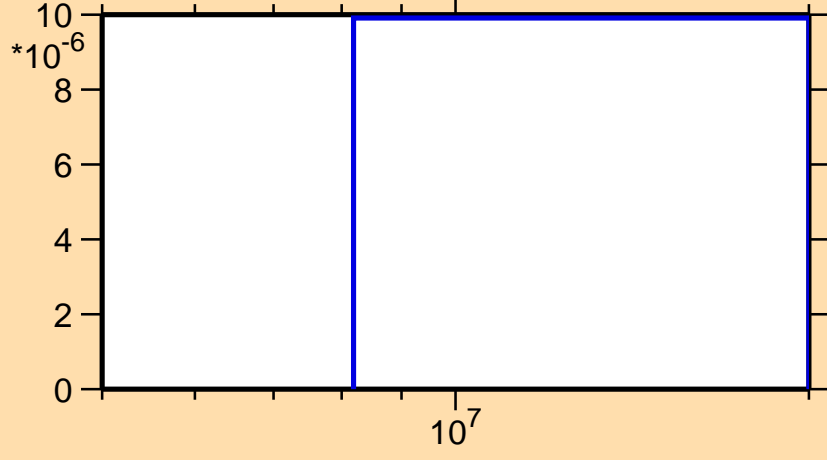
\sigma vs. E for ^{103}\text{Sn}(n,\text{pt})
