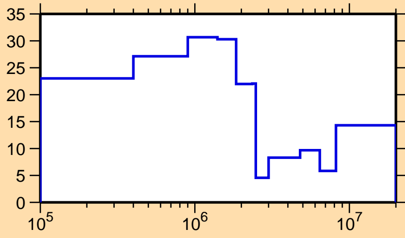
\Delta\sigma/\sigma vs. E for ^{103}\text{Sn}(n,\text{tot.})
