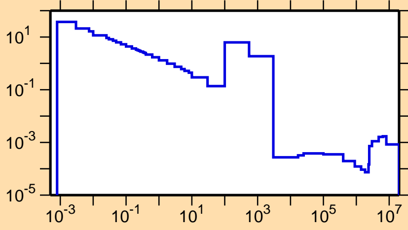
\sigma vs. E for ^{103}\text{Sn}(n,\gamma)
