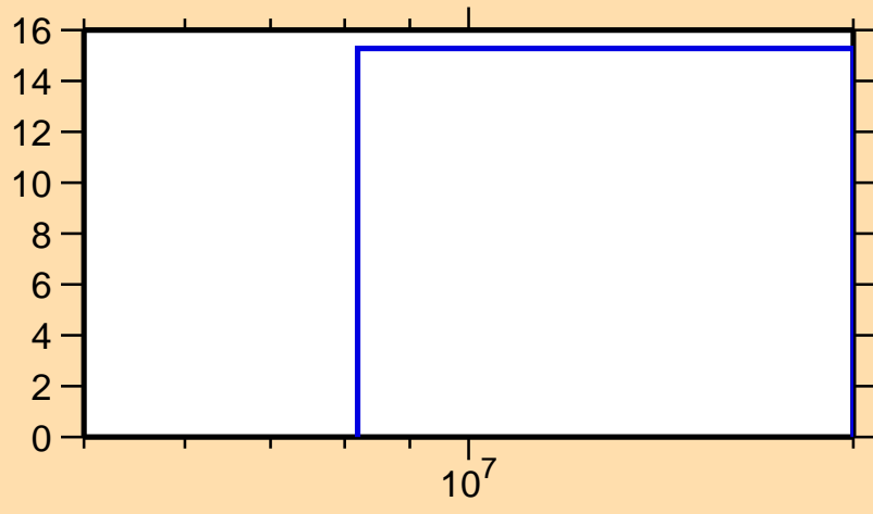
\Delta\sigma/\sigma vs. E for ^{103}\text{Sn}(n,\text{nonel.})
