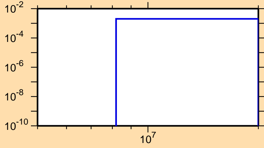
\sigma vs. E for ^{103}\text{Sn}(n,\text{pd})
