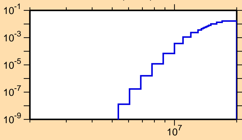
\sigma vs. E for ^{104}\text{Sn}(n,n\alpha)
