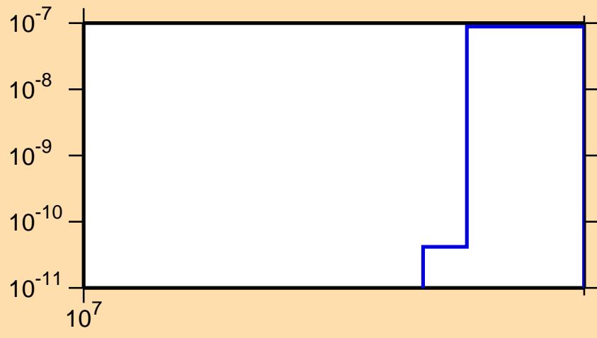
\sigma vs. E for ^{104}\text{Sn}(n,\text{nd})
