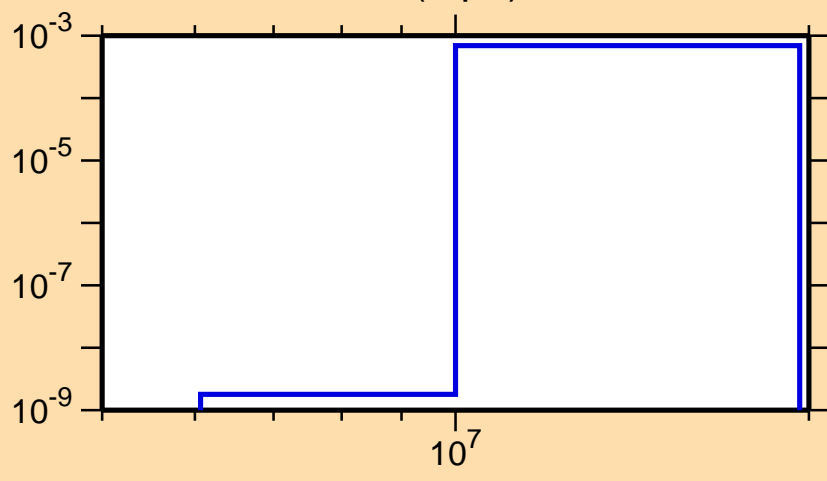
\sigma vs. E for ^{104}\text{Sn}(n,\text{pd})
