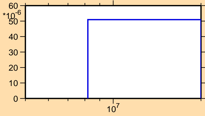
\sigma vs. E for ^{104}\text{Sn}(n,t)
