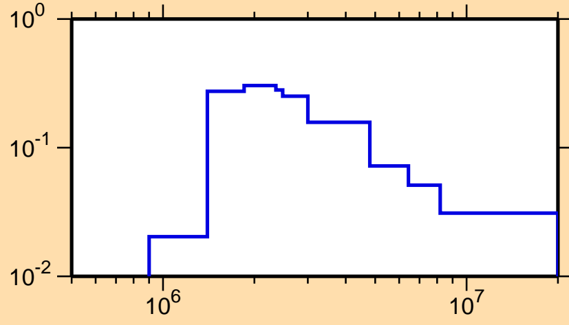
\sigma vs. E for ^{104}\text{Sn}(n,n_1)
