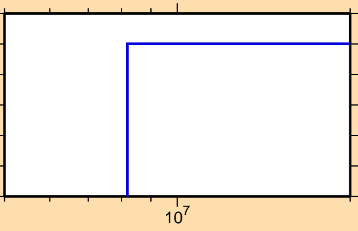
\sigma vs. E for ^{104}\text{Sn}(n,2np)
