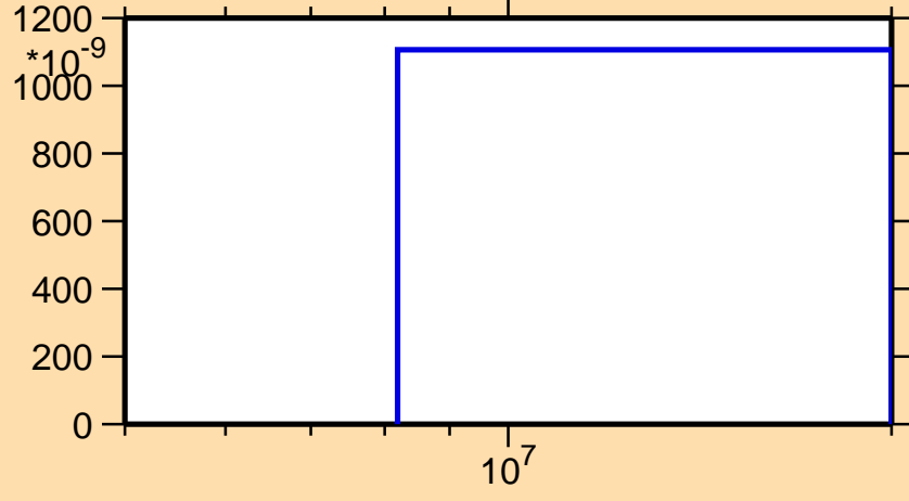
\sigma vs. E for ^{104}\text{Sn}(\text{mt } 45)
