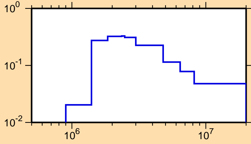
\sigma vs. E for ^{104}\text{Sn}(n,\text{inel.})
