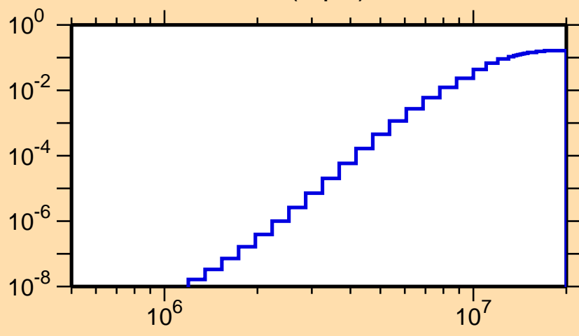
\sigma vs. E for ^{105}\text{Sn}(n,p\alpha)
