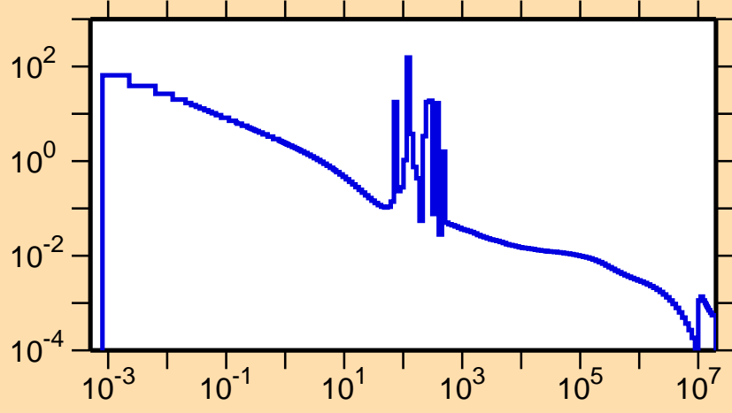
\sigma vs. E for ^{105}\text{Sn}(n,\gamma)
