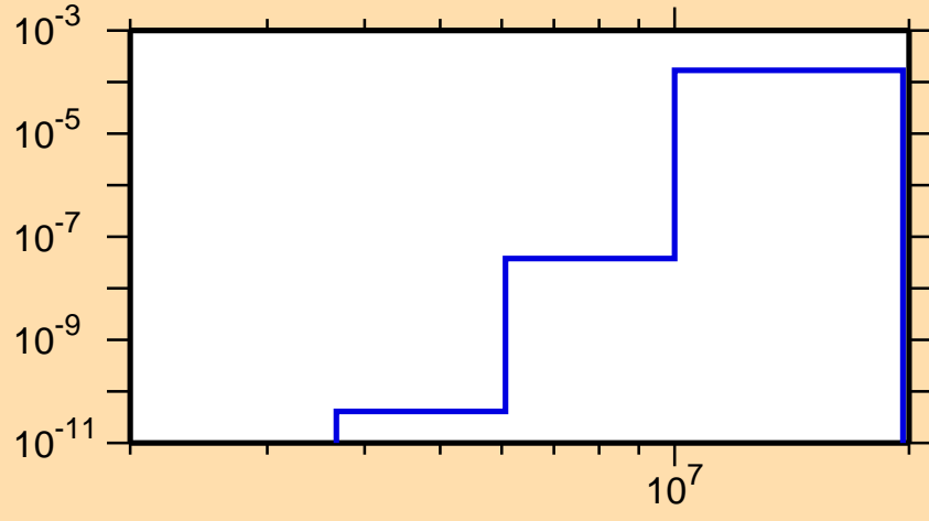
\sigma vs. E for ^{105}\text{Sn}(n,\text{He}3)
