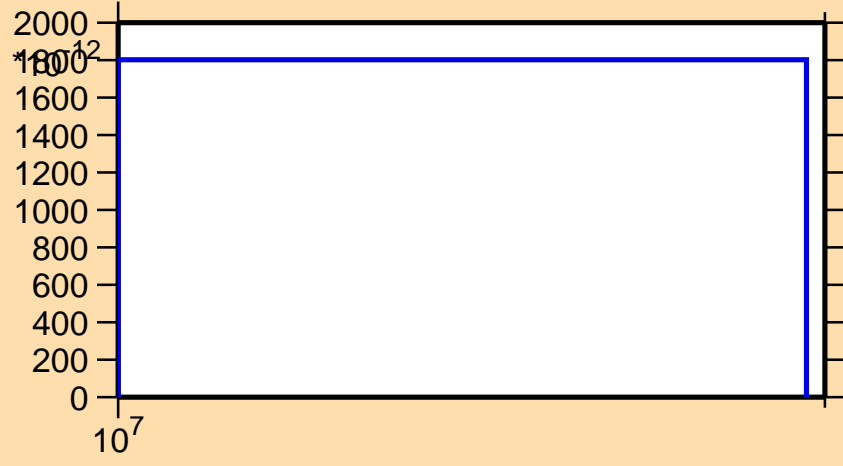
\sigma vs. E for ^{105}\text{Sn} (mt 34)
