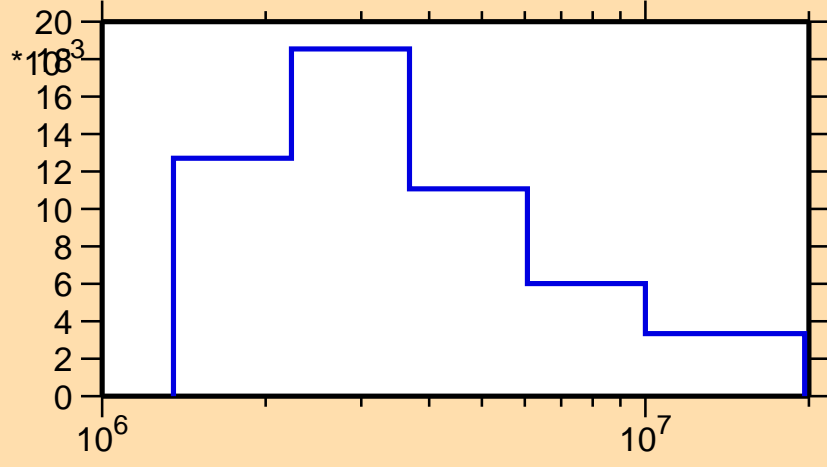
\sigma vs. E for ^{105}\text{Sn}(n,n_3)
