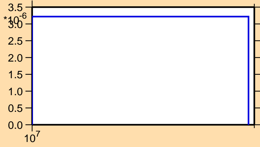
\sigma vs. E for ^{105}\text{Sn}(n,2np)
