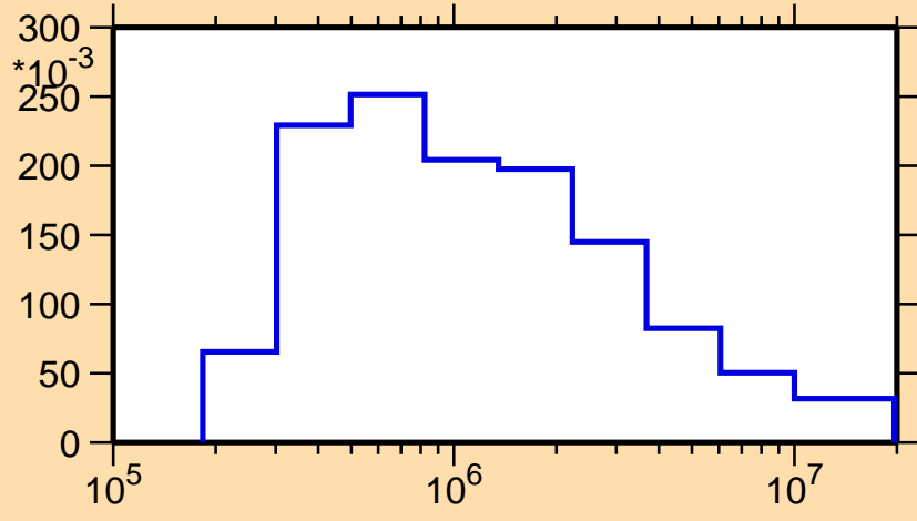
\sigma vs. E for ^{105}\text{Sn}(n,\text{inel.})
