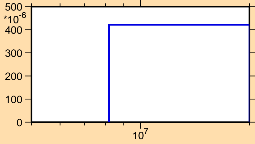
\sigma vs. E for ^{105}\text{Sn}(n,\text{pd})
