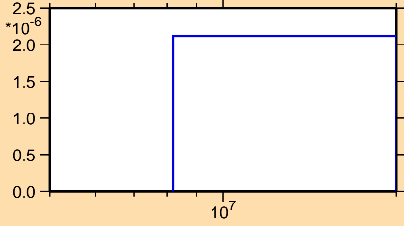
\sigma vs. E for ^{105}\text{Sn}(n,\text{pt})
