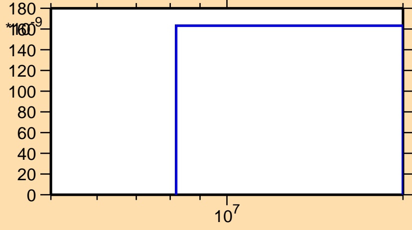
\sigma vs. E for ^{105}\text{Sn}(n,nd)
