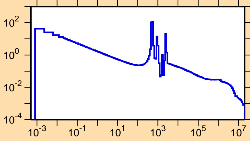
\sigma vs. E for ^{106}\text{Sn}(n,\gamma)
