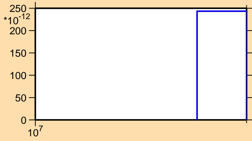
\sigma vs. E for ^{106}\text{Sn} (mt 34)
