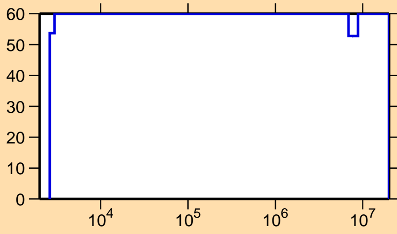
\Delta\sigma/\sigma vs. E for ^{106}\text{Sn}(n,\gamma)
