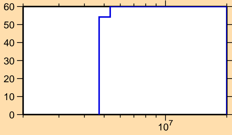
\Delta\sigma/\sigma vs. E for ^{106}\text{Sn}(n,n\text{cont.})
