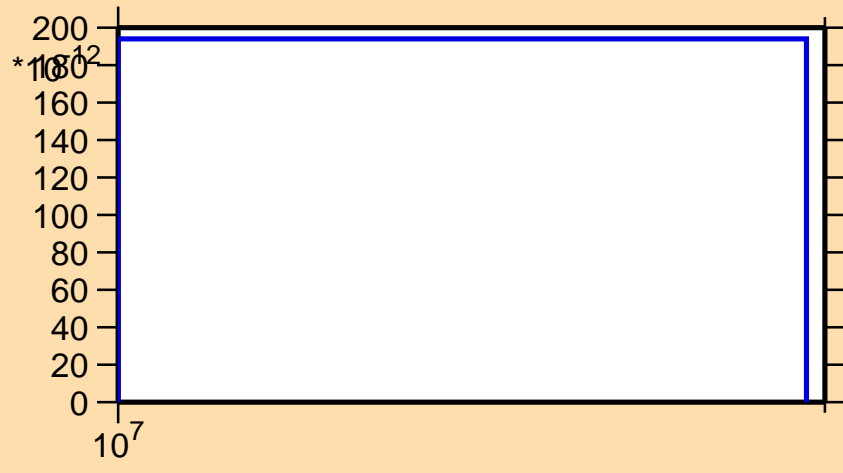
\sigma vs. E for ^{107}\text{Sn} (mt 34)
