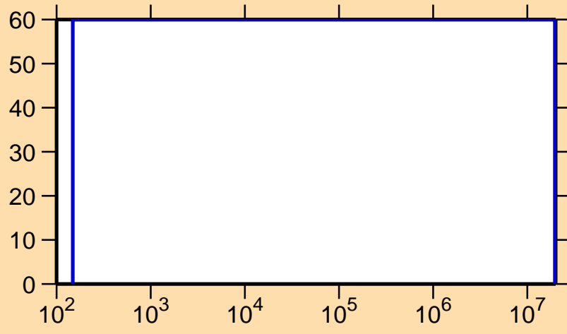
\Delta\sigma/\sigma vs. E for ^{107}\text{Sn}(n,\gamma)
