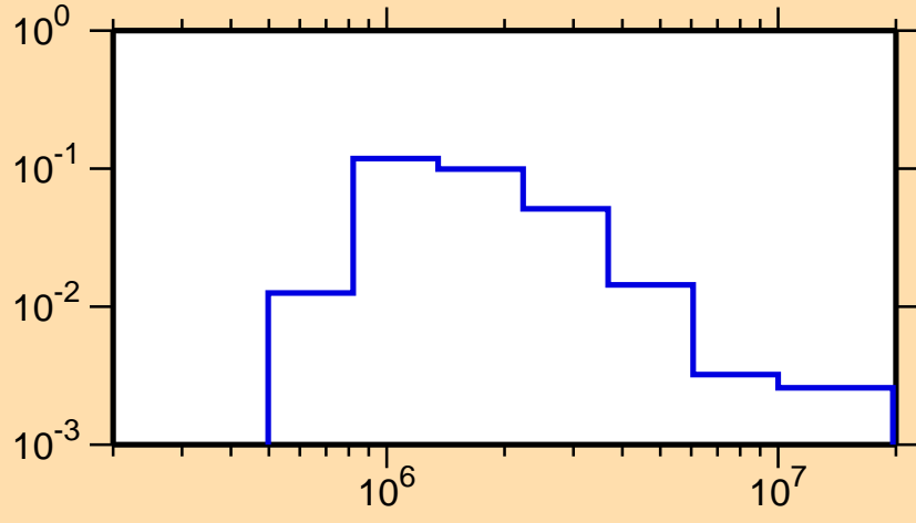
\sigma vs. E for ^{107}\text{Sn}(n,n_2)
