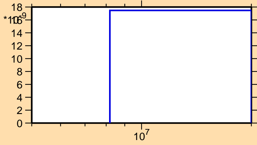
\sigma vs. E for ^{107}\text{Sn}(\text{mt117})
