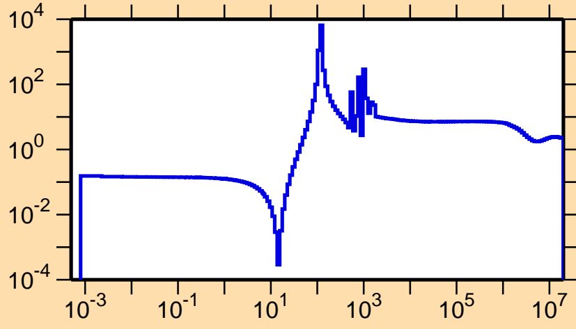
\sigma vs. E for ^{108}\text{Sn}(n,\text{el.})
