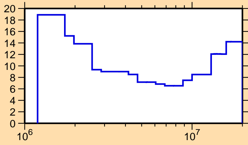
\Delta\sigma/\sigma vs. E for ^{108}\text{Sn}(n,\text{tot.})
