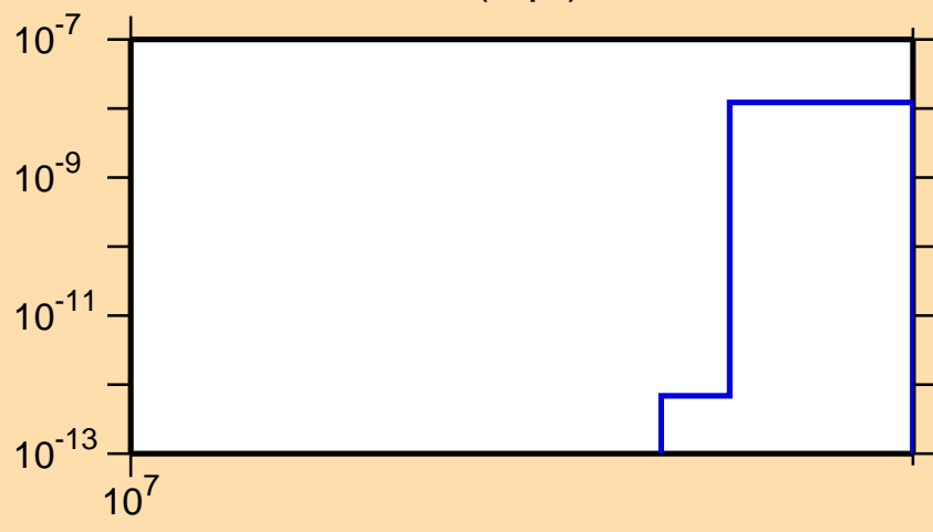
\sigma vs. E for ^{108}\text{Sn}(n,\text{pt})
