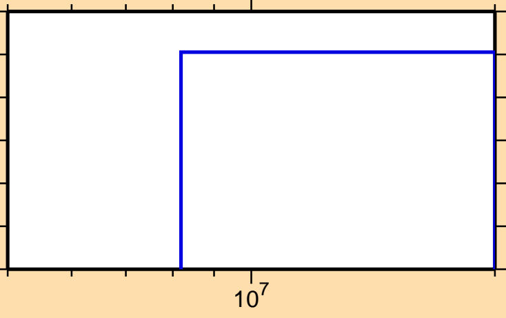
\sigma vs. E for ^{108}\text{Sn}(\text{mt117})
