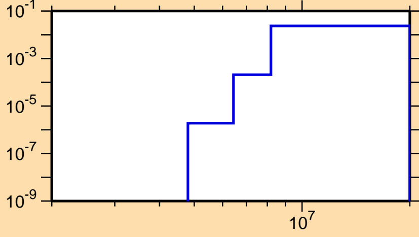
\sigma vs. E for ^{108}\text{Sn}(n,n\alpha)
