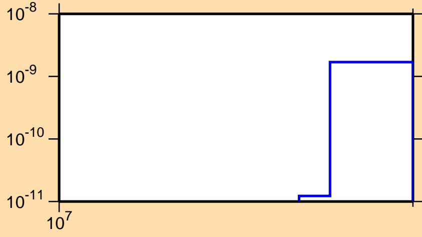
\sigma vs. E for ^{109}\text{Sn} (mt 34)
