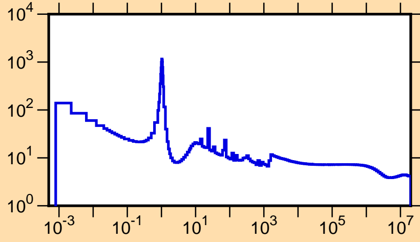
\sigma vs. E for ^{109}\text{Sn}(n,\text{tot.})
