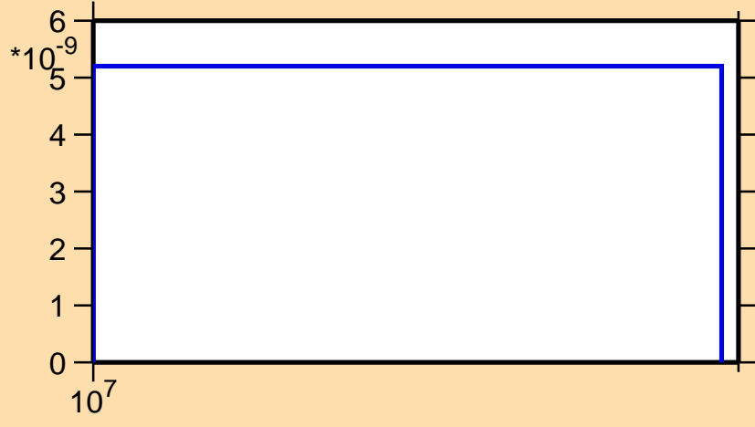
\sigma vs. E for ^{109}\text{Sn} (mt 45)
