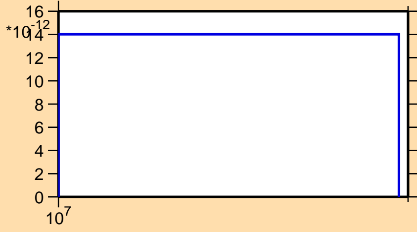
\sigma vs. E for ^{109}\text{Sn} (mt 34)
