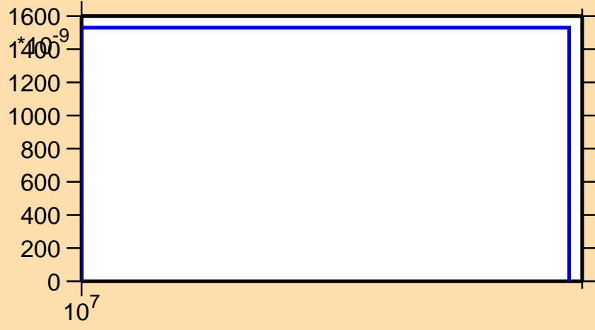
\sigma vs. E for ^{109}\text{Sn}(n,2n\alpha)
