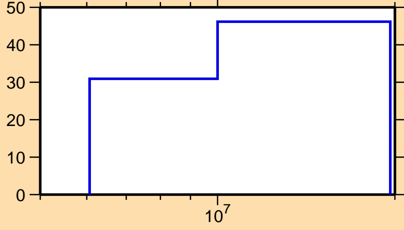
\Delta\sigma/\sigma vs. E for ^{109}\text{Sn}(n,\text{inel.})
