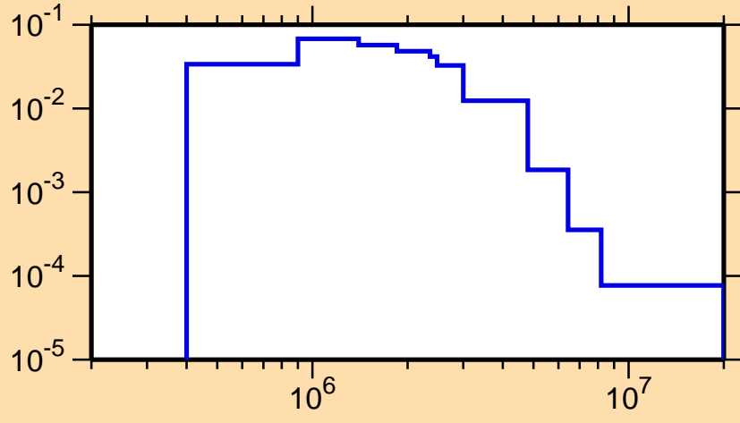
\sigma vs. E for ^{109}\text{Sn}(n,n_2)
