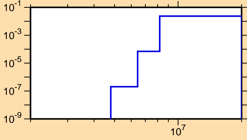
\sigma vs. E for ^{109}\text{Sn}(n,n\alpha)
