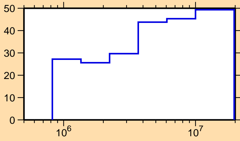
\Delta\sigma/\sigma vs. E for ^{110}\text{Sn}(n,n_1)
