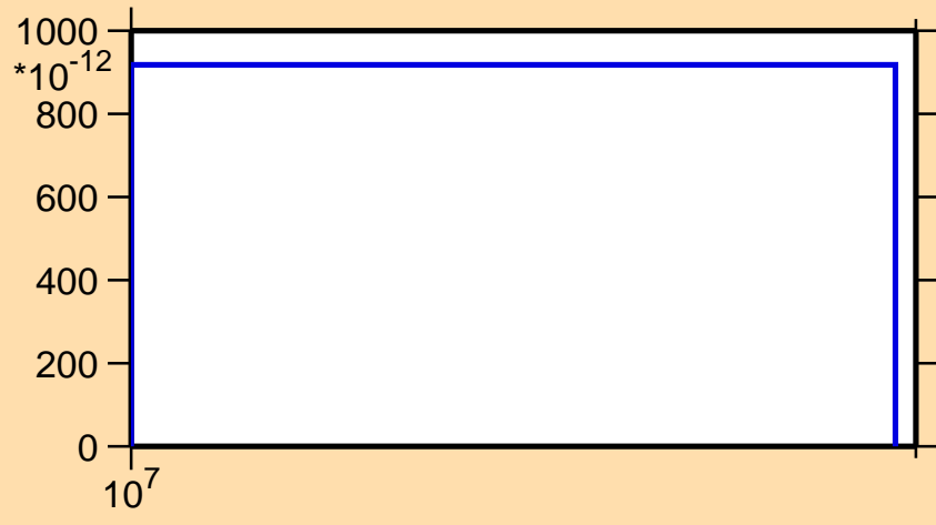
\sigma vs. E for ^{110}\text{Sn}(n,\text{nd})
