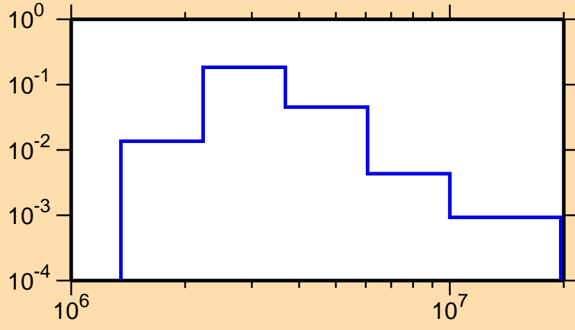
\sigma vs. E for ^{110}\text{Sn}(n,n_2)
