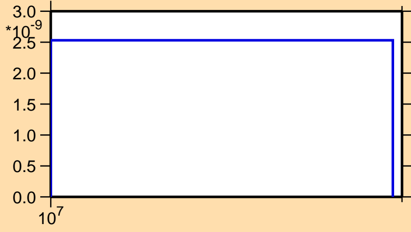
\sigma vs. E for ^{110}\text{Sn}(n,2n\alpha)
