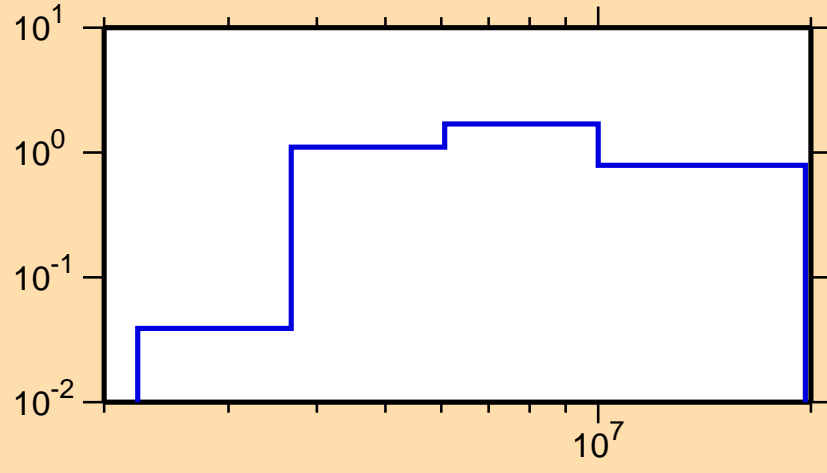
\sigma vs. E for ^{110}\text{Sn}(n,n\text{cont.})
