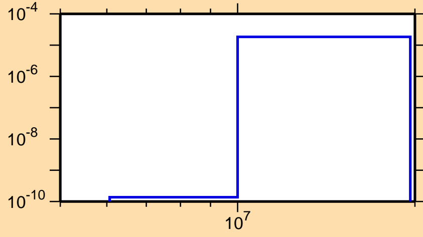
\sigma vs. E for ^{110}\text{Sn}(n,p\alpha)
