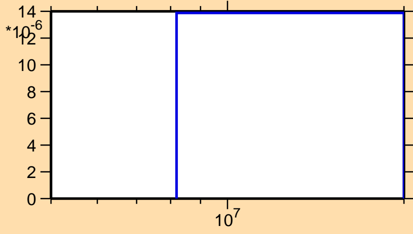
\sigma vs. E for ^{110}\text{Sn}(n,t)
