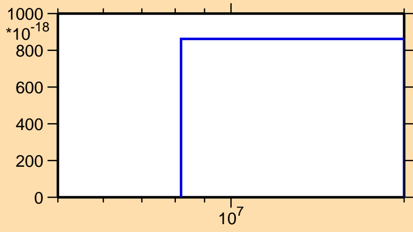
\sigma vs. E for ^{110}\text{Sn}(n,nt)
