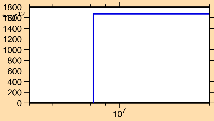
\sigma vs. E for ^{110}\text{Sn}(n,2np)
