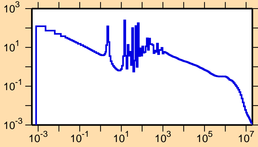
\sigma vs. E for ^{111}\text{Sn}(n,\gamma)
