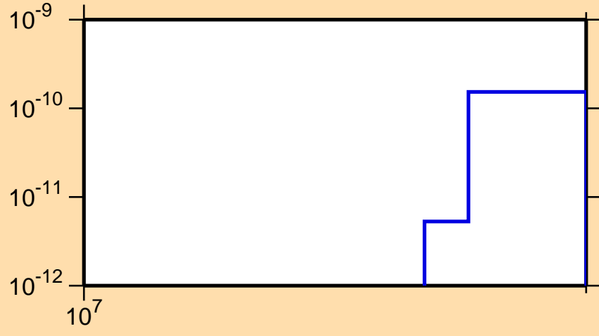
\sigma vs. E for ^{111}\text{Sn}(\text{mt117})
