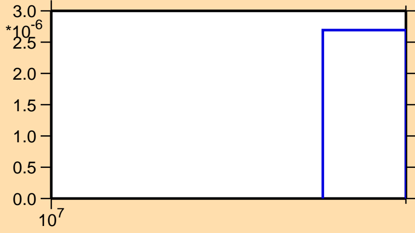
\sigma vs. E for ^{111}\text{Sn}(n,3n)
