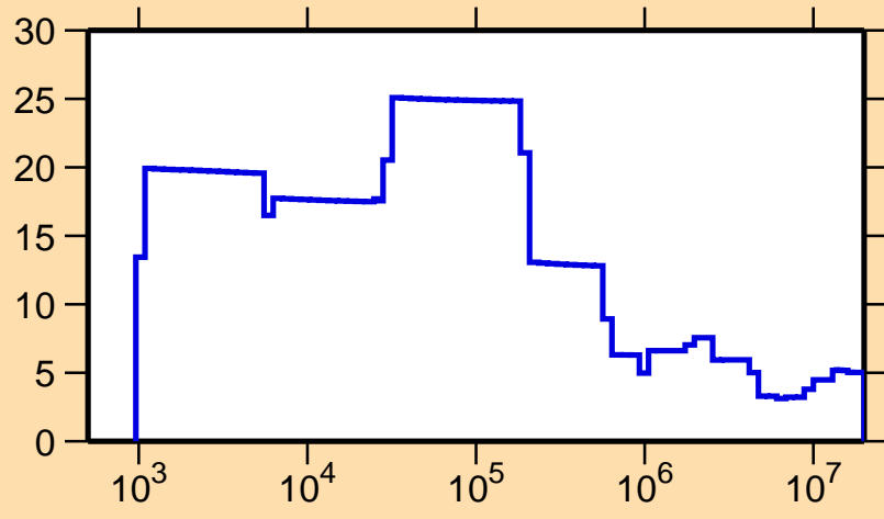
\Delta\sigma/\sigma vs. E for ^{111}\text{Sn}(n,\text{tot.})
