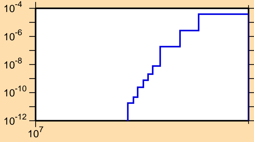
\sigma vs. E for ^{111}\text{Sn}(n,2n\alpha)
