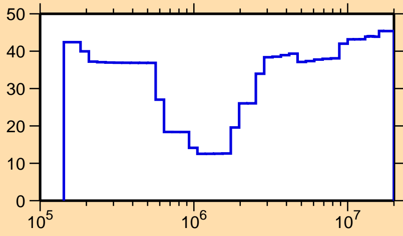
\Delta\sigma/\sigma vs. E for ^{111}\text{Sn}(n,n_1)
