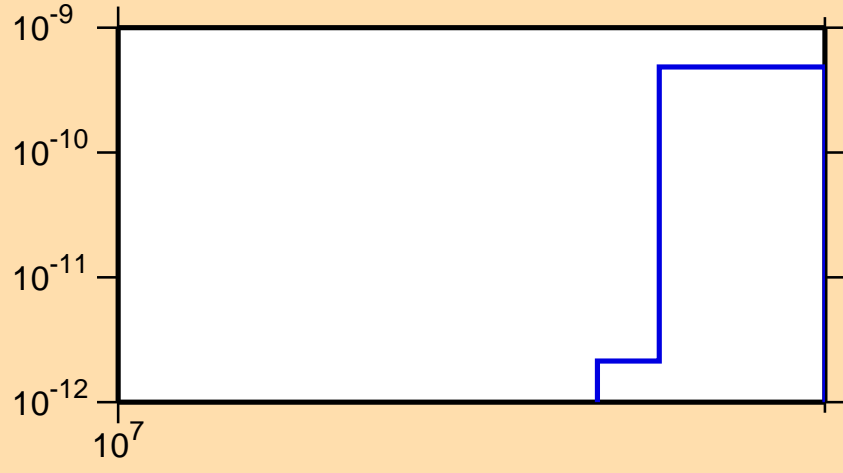
\sigma vs. E for ^{111}\text{Sn} (mt 45)
