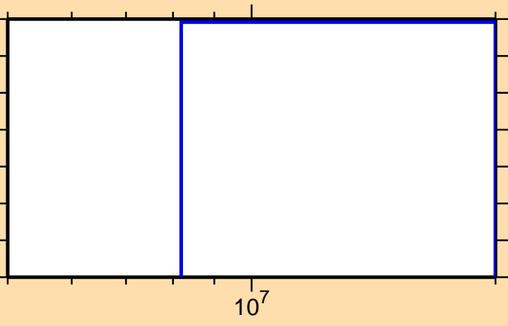
\sigma vs. E for ^{111}\text{Sn}(n,\text{He}3)
