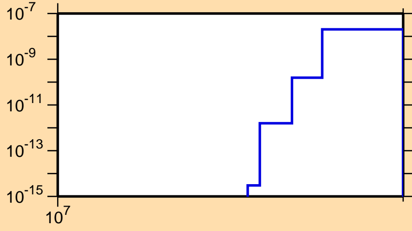
\sigma vs. E for ^{112}\text{Sn}(n,pd)
