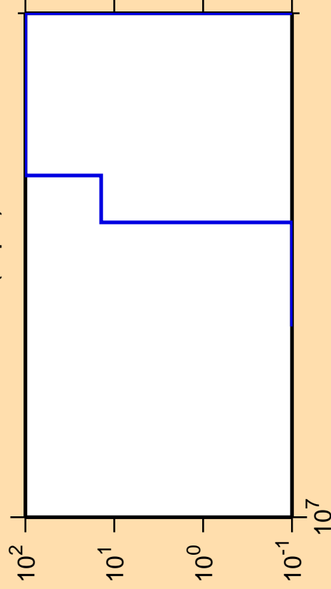
\Delta\sigma/\sigma vs. E for ^{112}\text{Sn}(n,pd)
