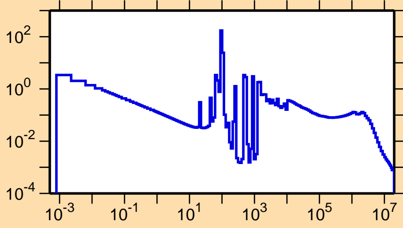
\sigma vs. E for ^{112}\text{Sn}(n,\gamma)
