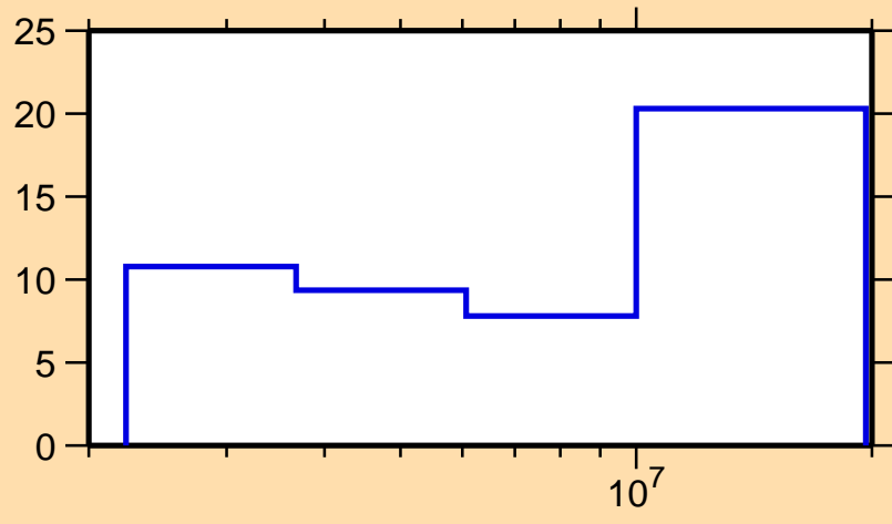
\Delta\sigma/\sigma vs. E for ^{112}\text{Sn}(n,n\text{cont.})
