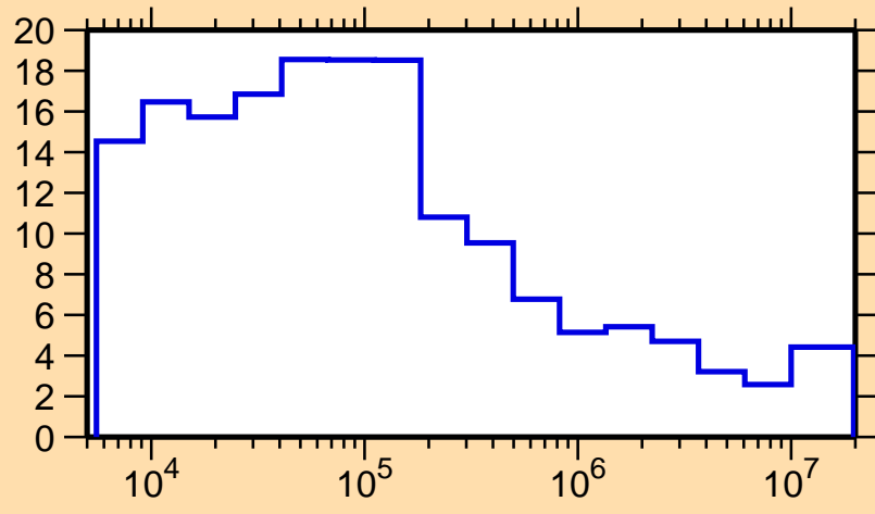
\Delta\sigma/\sigma vs. E for ^{112}\text{Sn}(n,\text{tot.})
