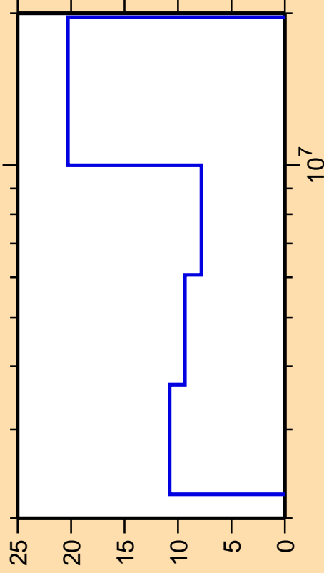
\Delta\sigma/\sigma vs. E for ^{112}\text{Sn}(n,n\text{cont.})
