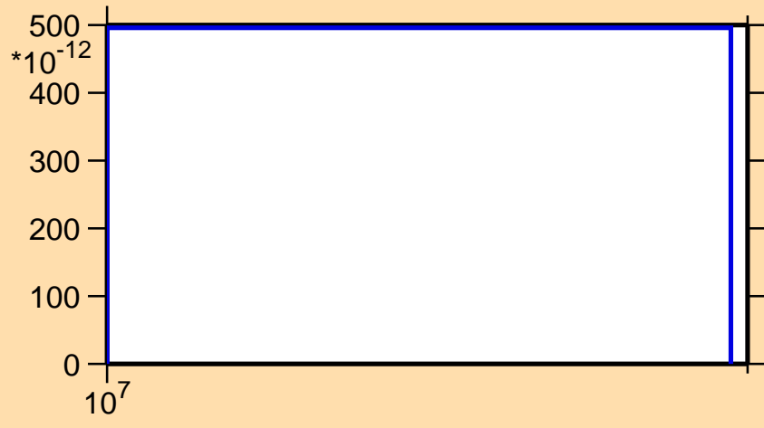
\sigma vs. E for ^{112}\text{Sn}(n,2n\alpha)
