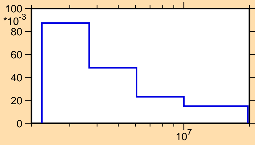
\sigma vs. E for ^{112}\text{Sn}(n,n_4)
