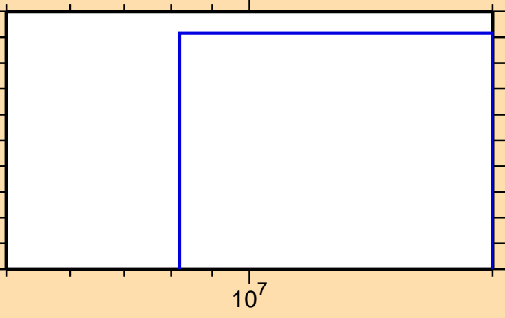
\sigma vs. E for ^{112}\text{Sn}(n,2np)
