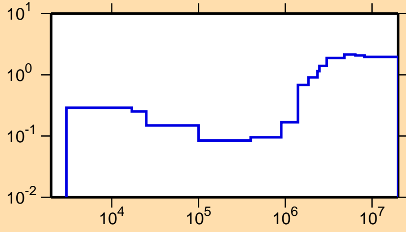
\sigma vs. E for ^{112}\text{Sn}(n,\text{nonel.})
