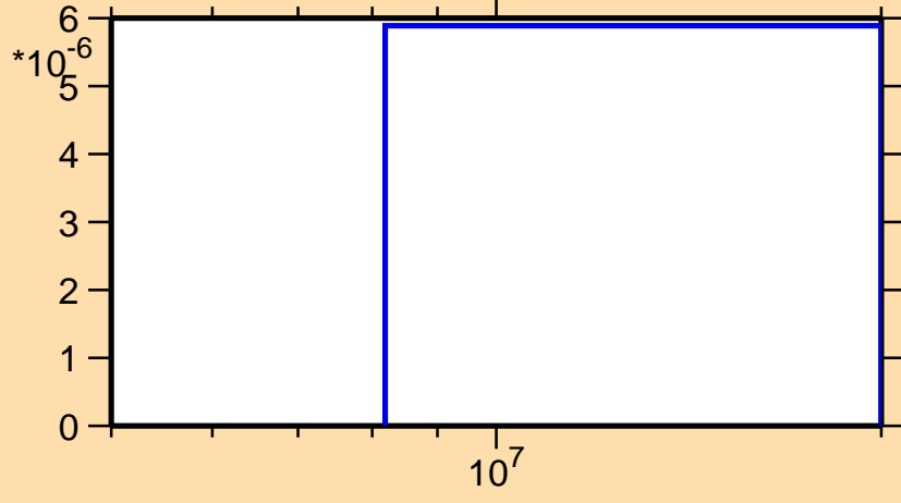
\sigma vs. E for ^{112}\text{Sn}(n,t)
