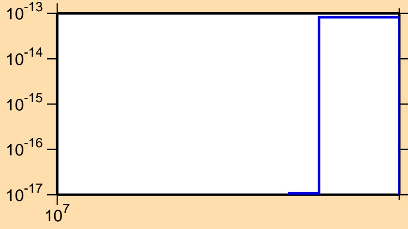
\sigma vs. E for ^{113}\text{Sn} (mt 45)
