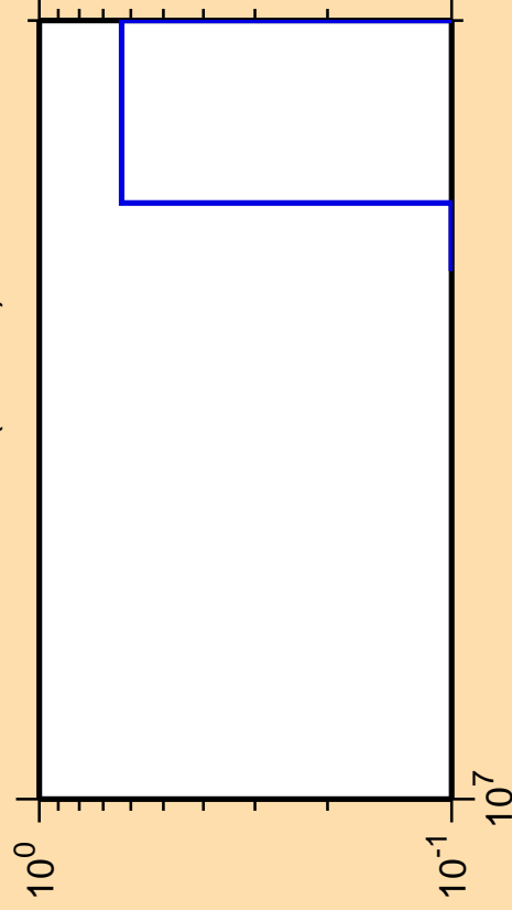
\Delta\sigma/\sigma vs. E for ^{113}\text{Sn} (mt 45)
